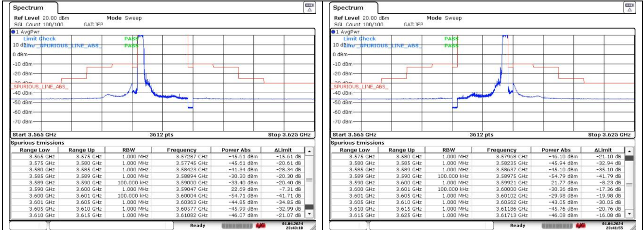
16QAM High Channel - 1 RB
