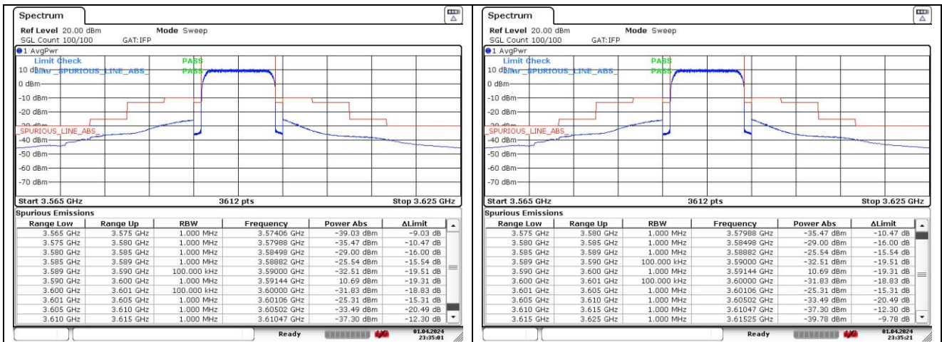
16QAM High Channel - Full RB
