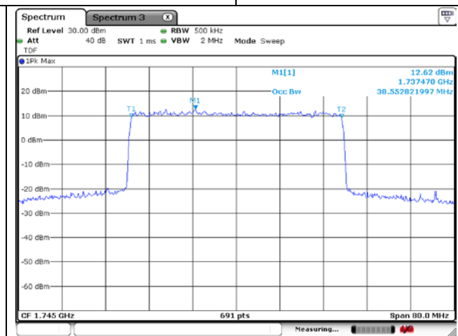
40 MHz CP-OFDM 16QAM
