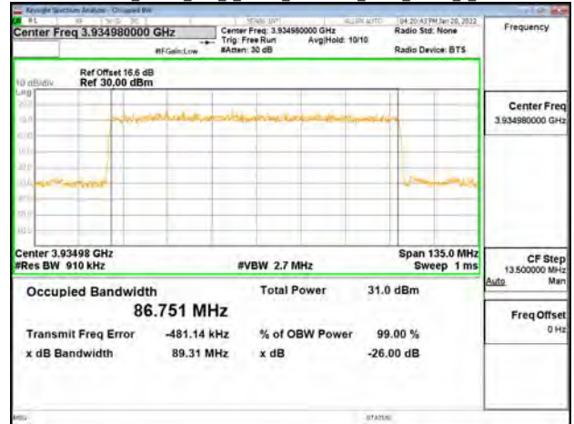
Band77-Part27_90MHz_DFT_s_OFDM_SCS30kHz_QPSK_RB243_0_CH649668
