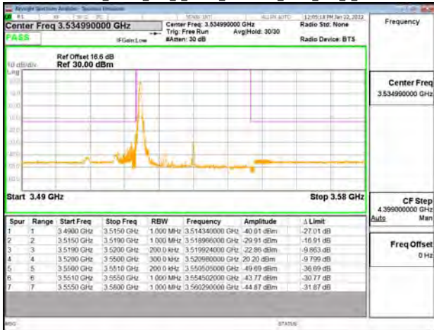
Band77-Part27_30MHz_DFT_s_OFDM_SCS30kHz_BPSK_RB1_0_CH635666
