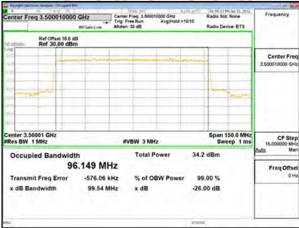
Band77-Part27_100MHz_DFT_s_OFDM_SCS30kHz_QPSK_RB270_0_CH633334
