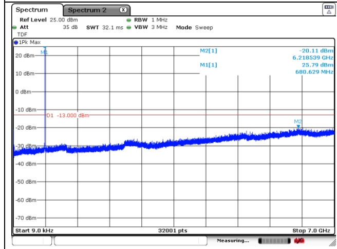
DFT-S-OFDM BPSK - 20 MHz Middle Channel - 1 RB
