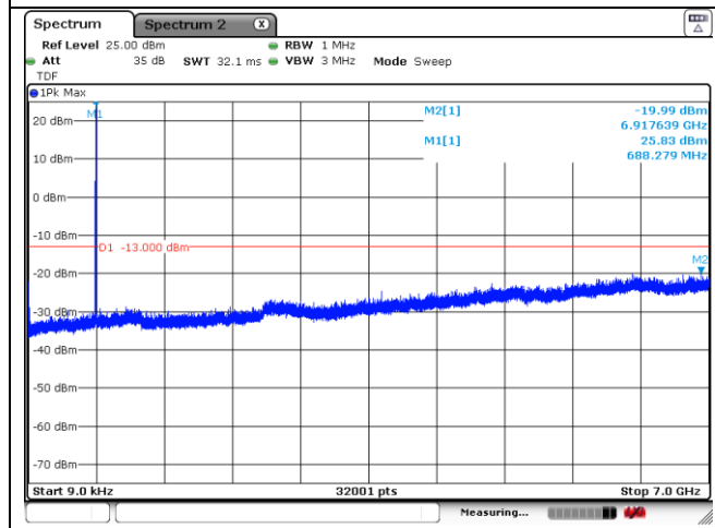
DFT-S-OFDM BPSK - 20 MHz High Channel - 1 RB
