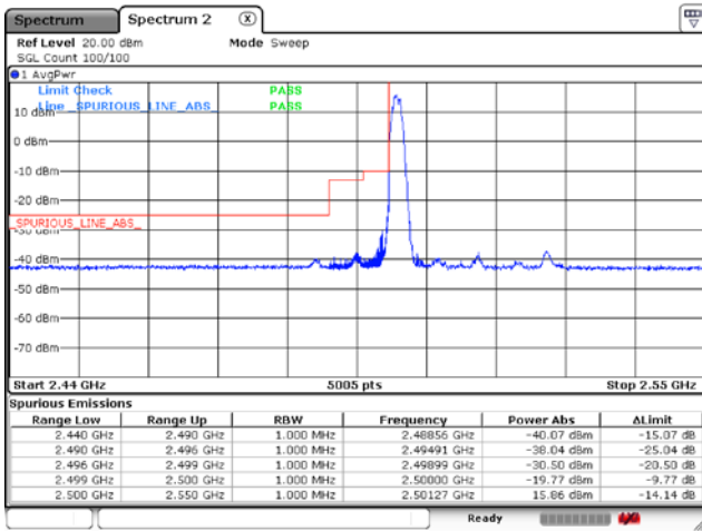
CP-OFDM 16QAM - IC Low Channel - 1 RB
