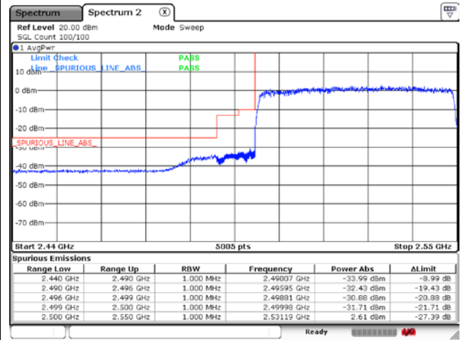
CP-OFDM 16QAM - IC Low Channel - Full RB
