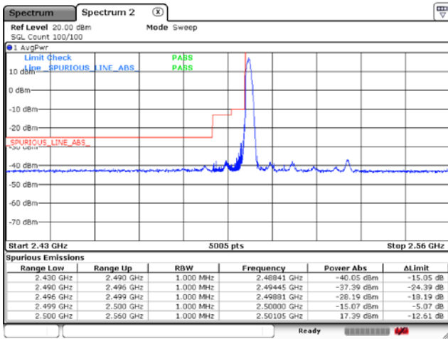
DFT-S-OFDM 16QAM - IC Low Channel - 1 RB
