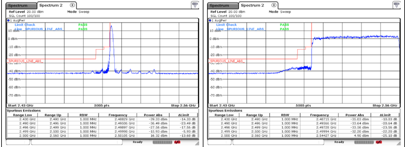
DFT-S-OFDM BPSK - IC Low Channel - 1 RB
