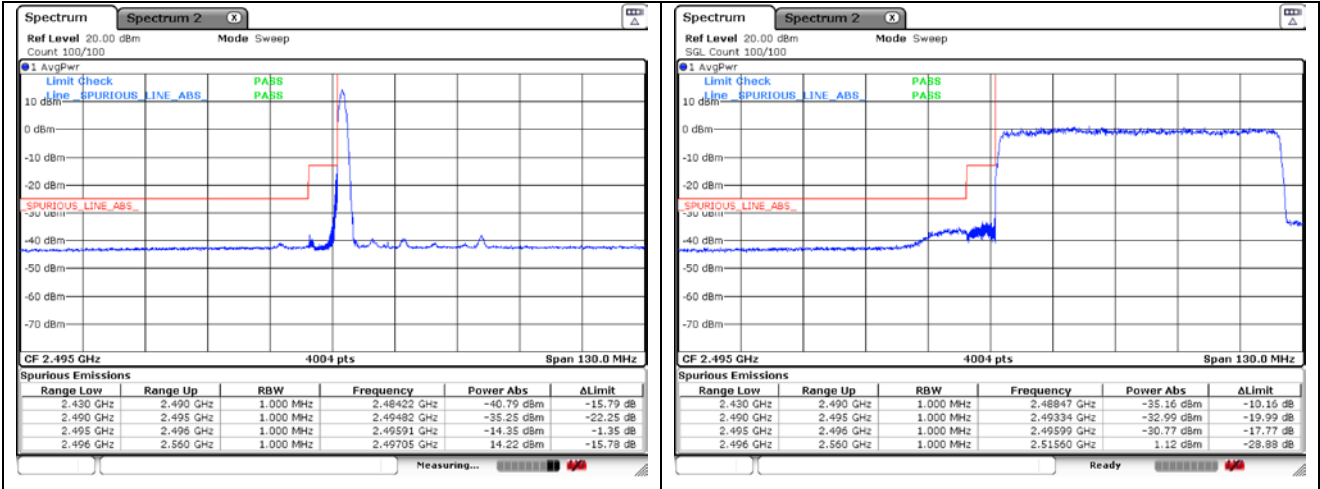
DFT-S-OFDM 16QAM - FCC Low Channel - 1 RB
