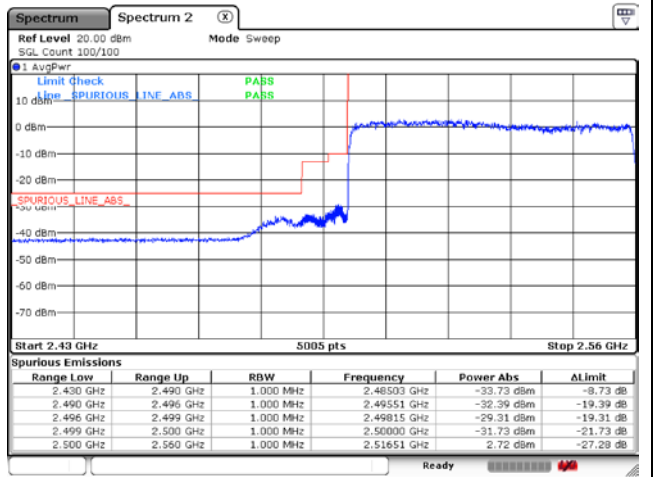
DFT-S-OFDM 16QAM - IC Low Channel - Full RB
