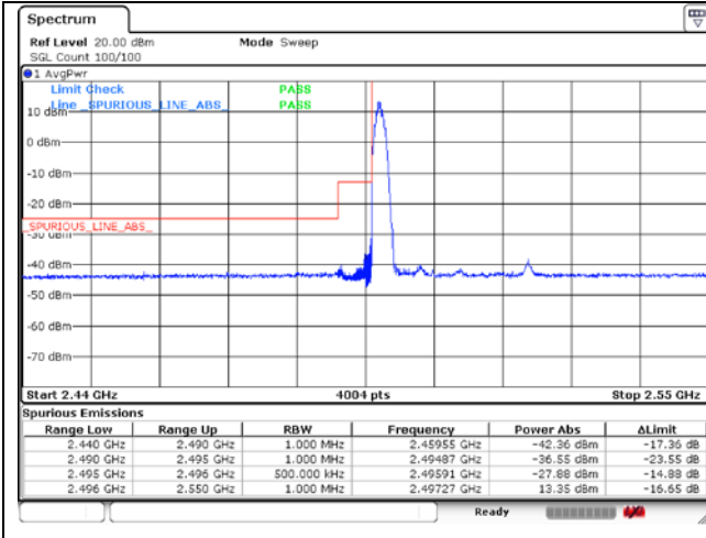
CP-OFDM QPSK - FCC Low Channel - 1 RB
