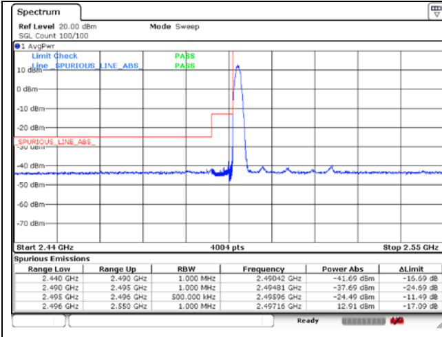
CP-OFDM 16QAM - FCC Low Channel - 1 RB
