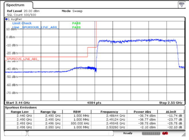
CP-OFDM QPSK - FCC Low Channel - Full RB
