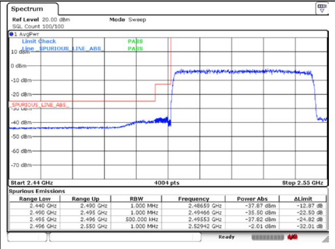
CP-OFDM 16QAM - FCC Low Channel - Full RB
