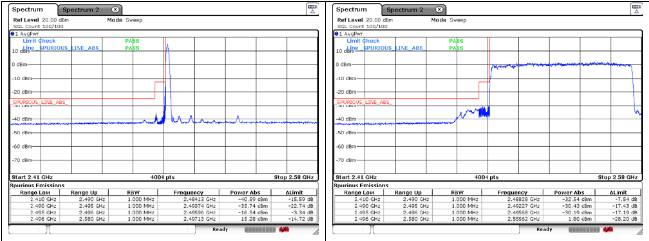
DFT-S-OFDM BPSK - FCC Low Channel - 1 RB
