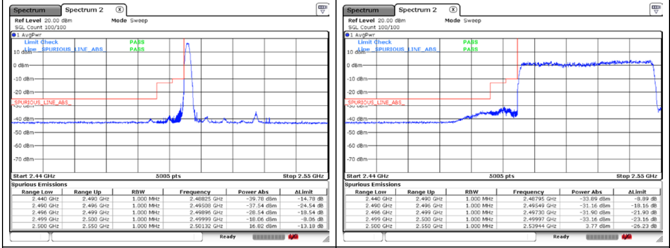
DFT-S-OFDM 16QAM - IC Low Channel - 1 RB
