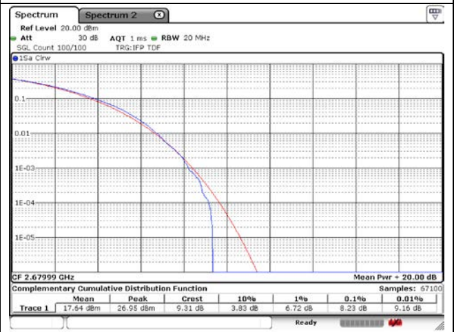
20 MHz High Channel - Full RB - CP-OFDM_Port 2
