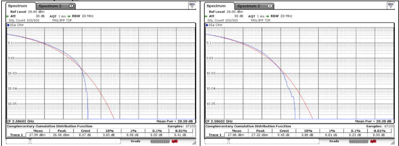
20 MHz Low Channel - Full RB - CP-OFDM_Port 1
