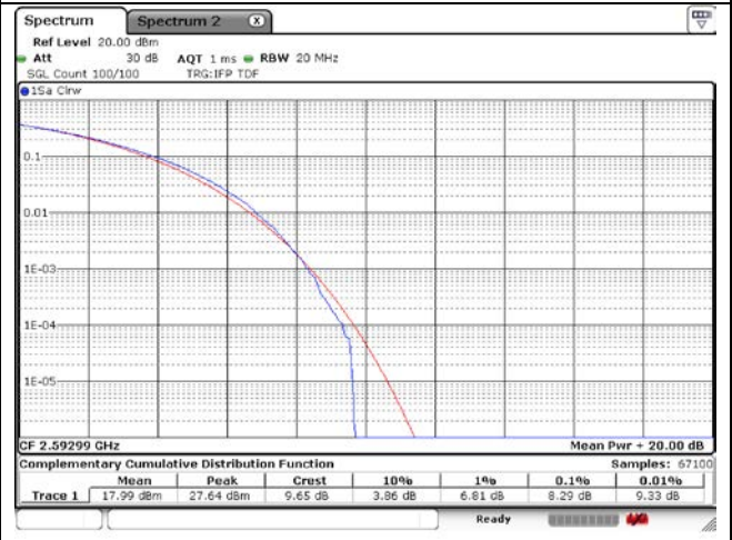
20 MHz Middle Channel - Full RB - CP-OFDM_Port 2
