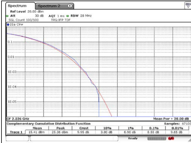
60 MHz Low Channel - Full RB - CP-OFDM_Port 1
