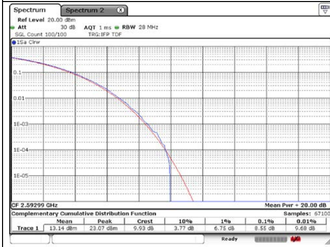
90 MHz Middle Channel - Full RB - CP-OFDM_Port 1
