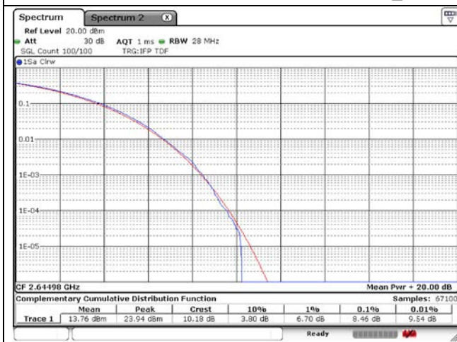
90 MHz High Channel - Full RB - CP-OFDM_Port 1
