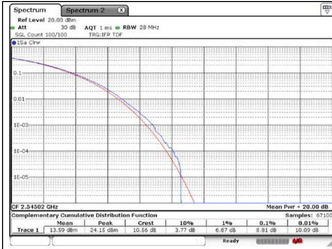
90 MHz Low Channel - Full RB - CP-OFDM_Port 1
