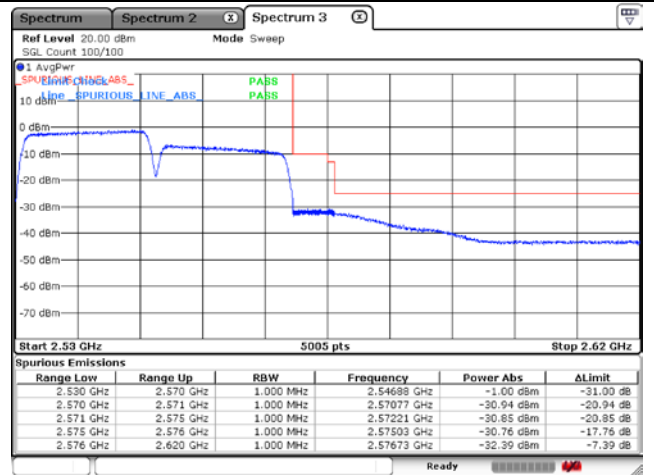
PCC 20 MHz + SCC 20 MHz_QPSK-High Channel
