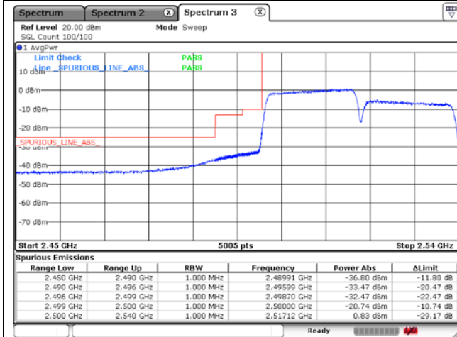
PCC 20 MHz + SCC 20 MHz_QPSK-Low Channel
