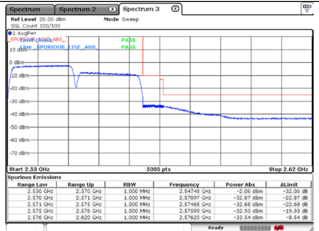
PCC 20 MHz + SCC 20 MHz_16QAM-High Channel
