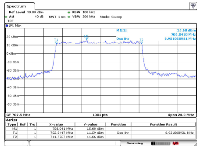
10 MHz DFT-S-OFDM QPSK
