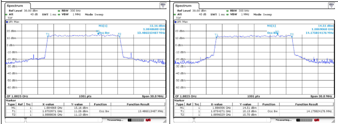
15 MHz DFT-S-OFDM 16QAM
