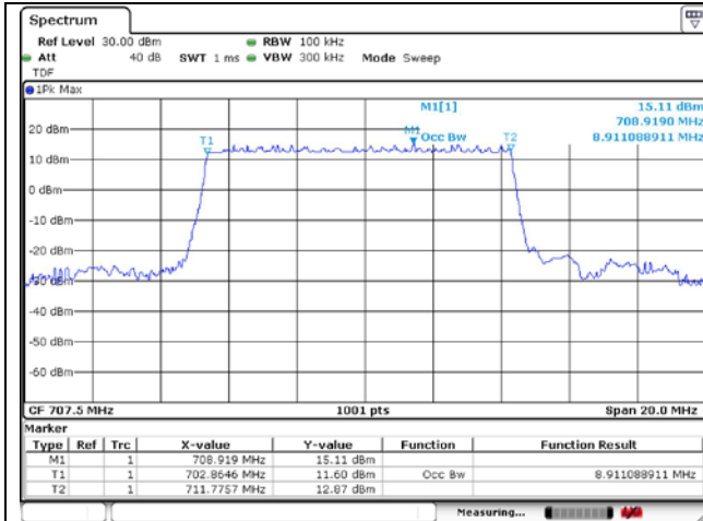
10 MHz DFT-S-OFDM BPSK
