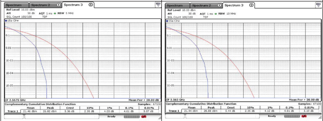
5 MHz QPSK High Channel - Full RB
