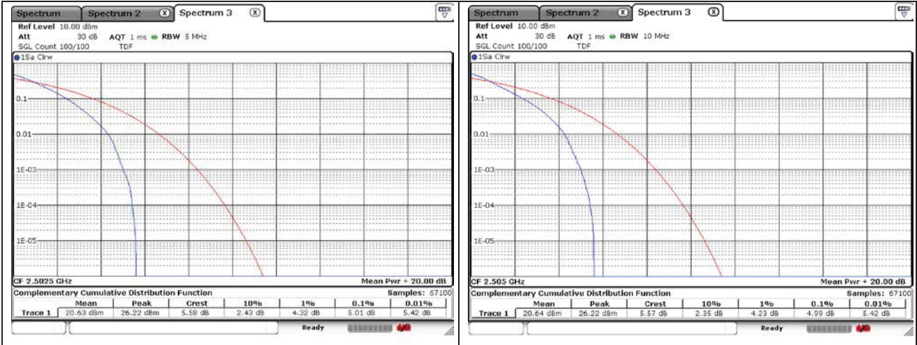
5 MHz QPSK Low Channel - Full RB
