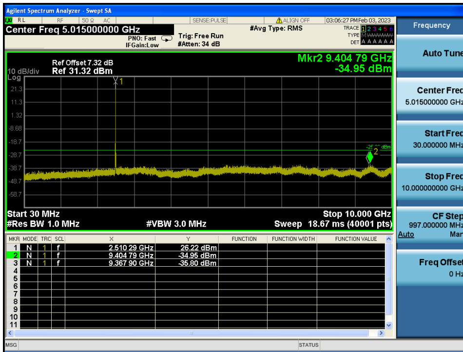
LTE Band 7 / 20 MHz / 16QAM - RB Size/Offset (1/50) – Low Channel
