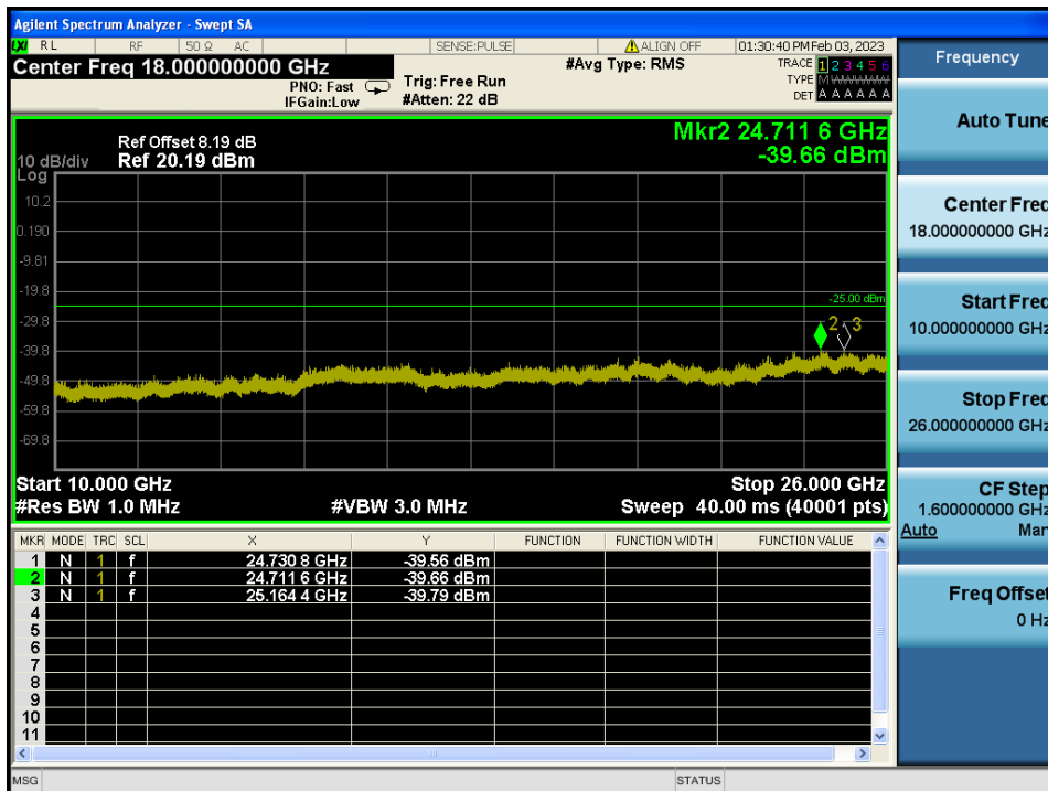
LTE Band 7 / 5 MHz / 16QAM - RB Size/Offset (1/12) – High Channel
