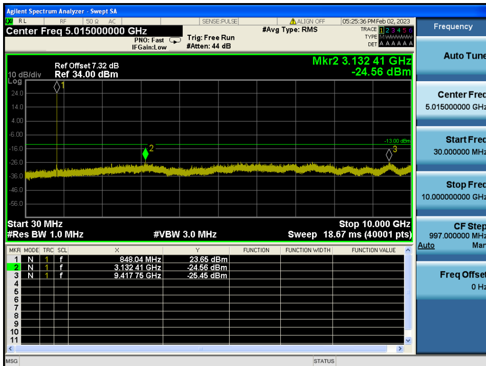
LTE Band 5 / 5 MHz / 16QAM - RB Size/Offset (12/13) – High Channel
