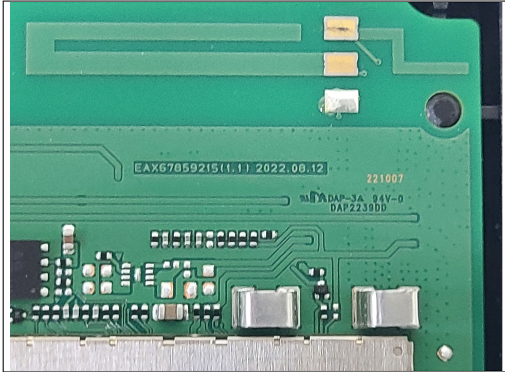
<Internal Antenna>
