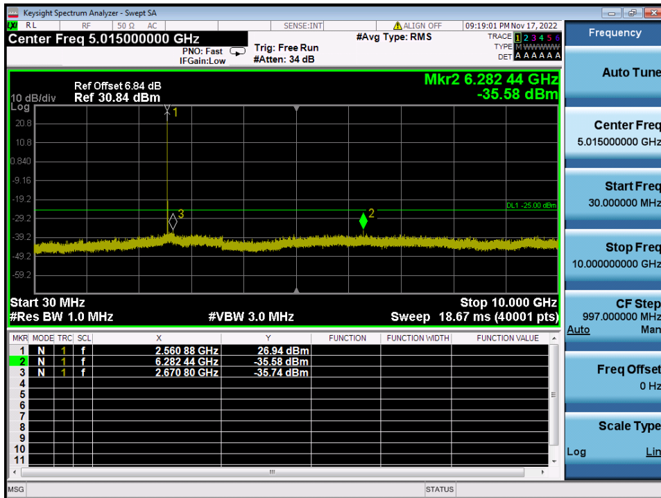
LTE Band 7 / 10 MHz / 16QAM - RB Size/Offset (1/0) – High Channel
