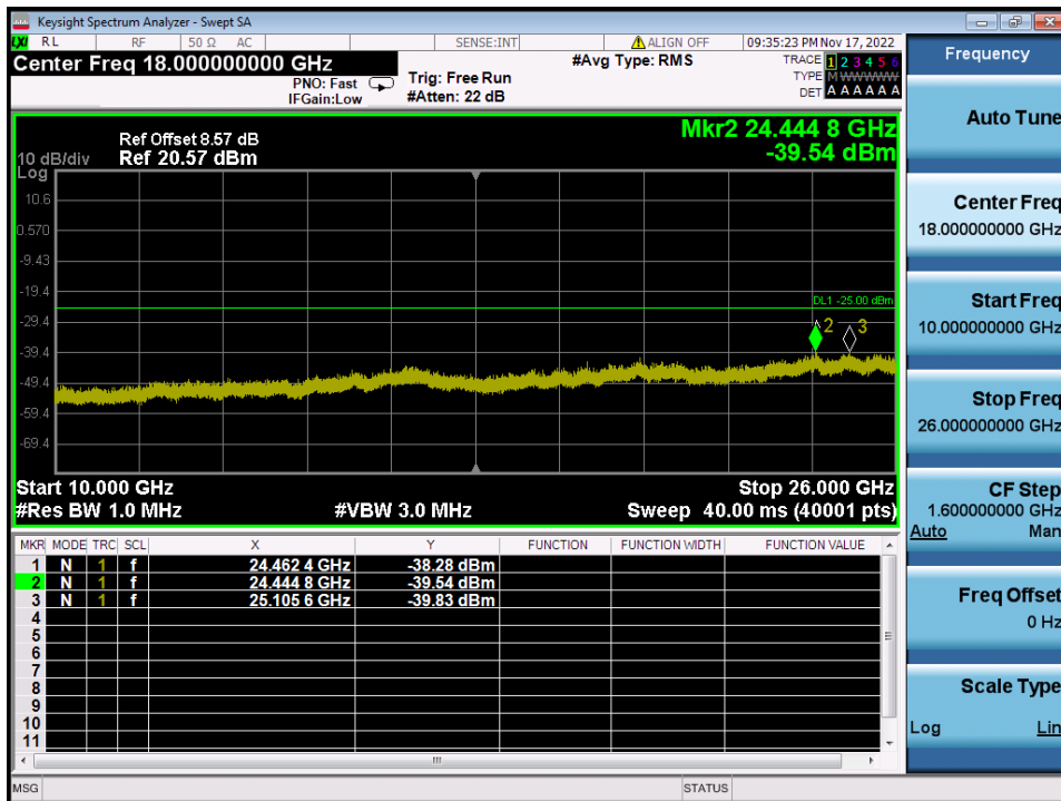
LTE Band 7 / 15 MHz / 16QAM - RB Size/Offset (36/18) – Low Channel
