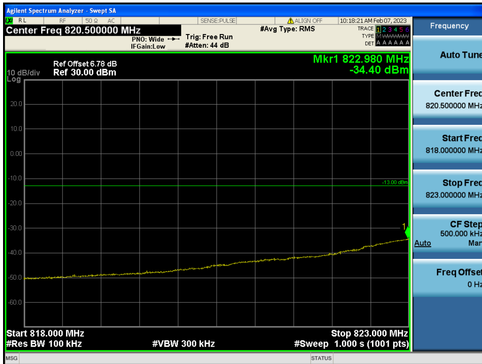
LTE Band 5 / 5 MHz / 16QAM - RB Size/Offset (12/0)
