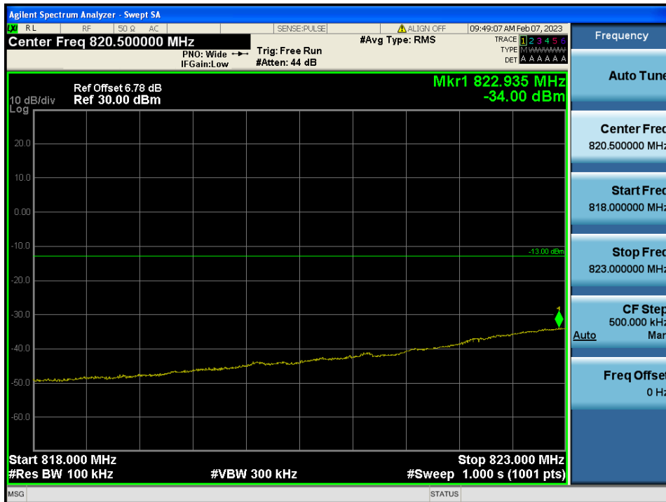
LTE Band 5 / 3 MHz / 16QAM - RB Size/Offset (15/0)
