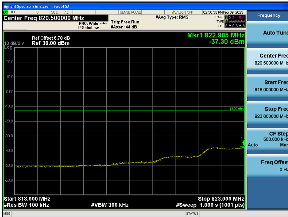
LTE Band 5 / 1.4 MHz / QPSK - RB Size/Offset (6/0)
