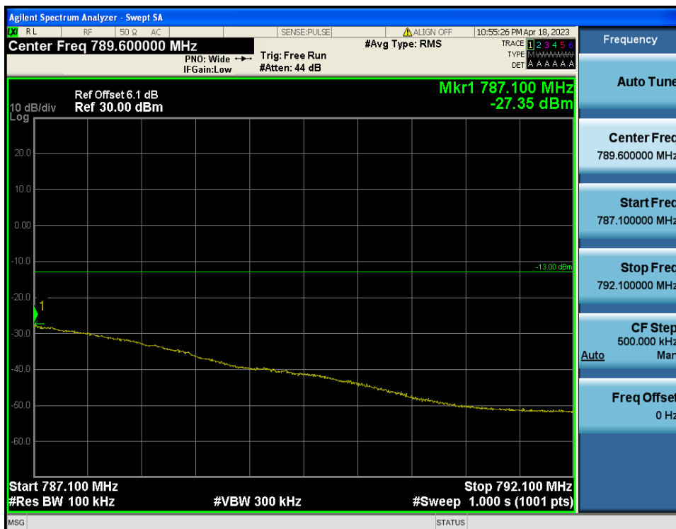
LTE Band 13 / 5MHz / 16QAM - RB Size/Offset (12/13)
