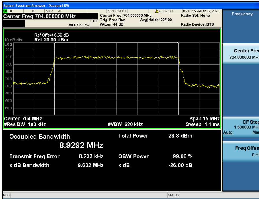
LTE Band 12 / 10MHz / QPSK - RB Size 50
