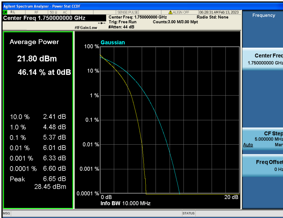
LTE Band 4 / 10MHz / QPSK - RB Size 50
