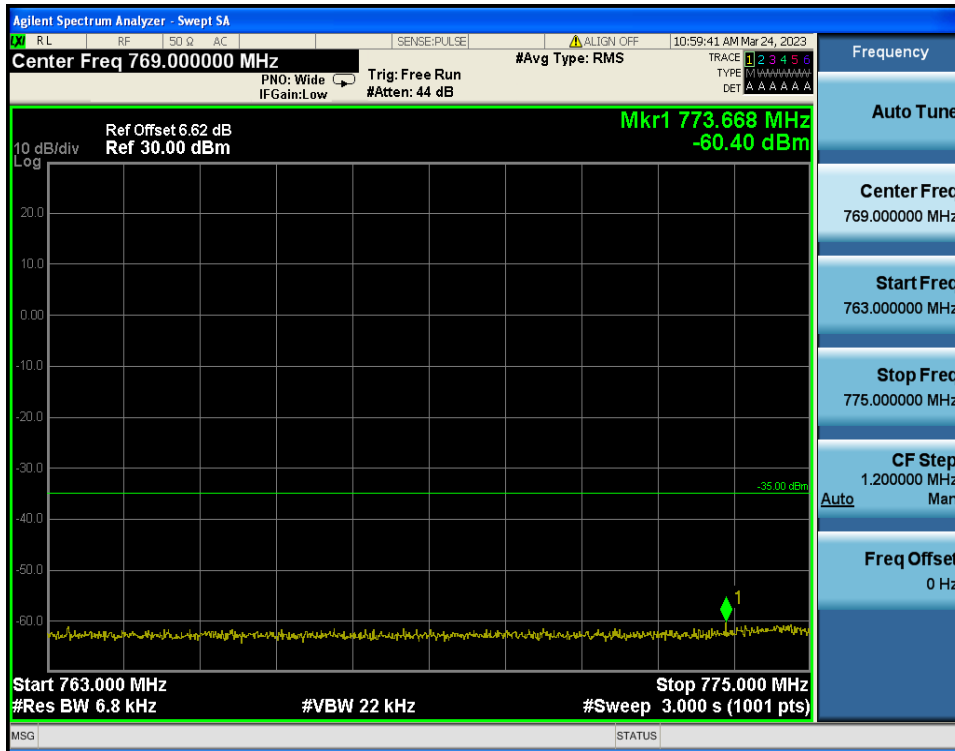
LTE Band 13 / 5 MHz / 16QAM - RB Size/Offset (25/0)
