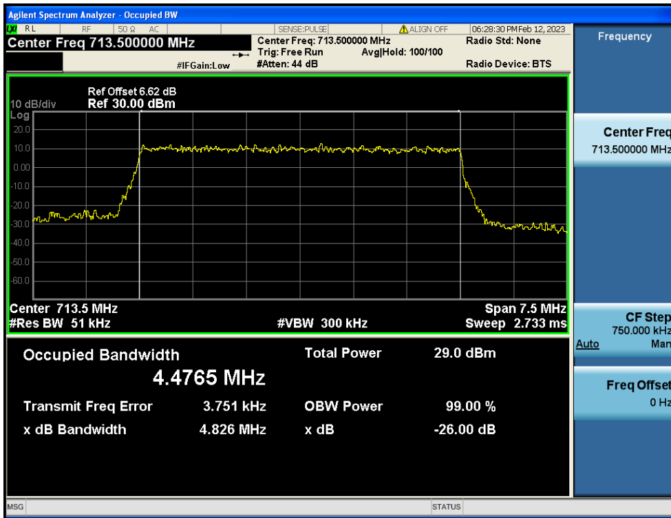
LTE Band 12 / 5MHz / QPSK - RB Size 25
