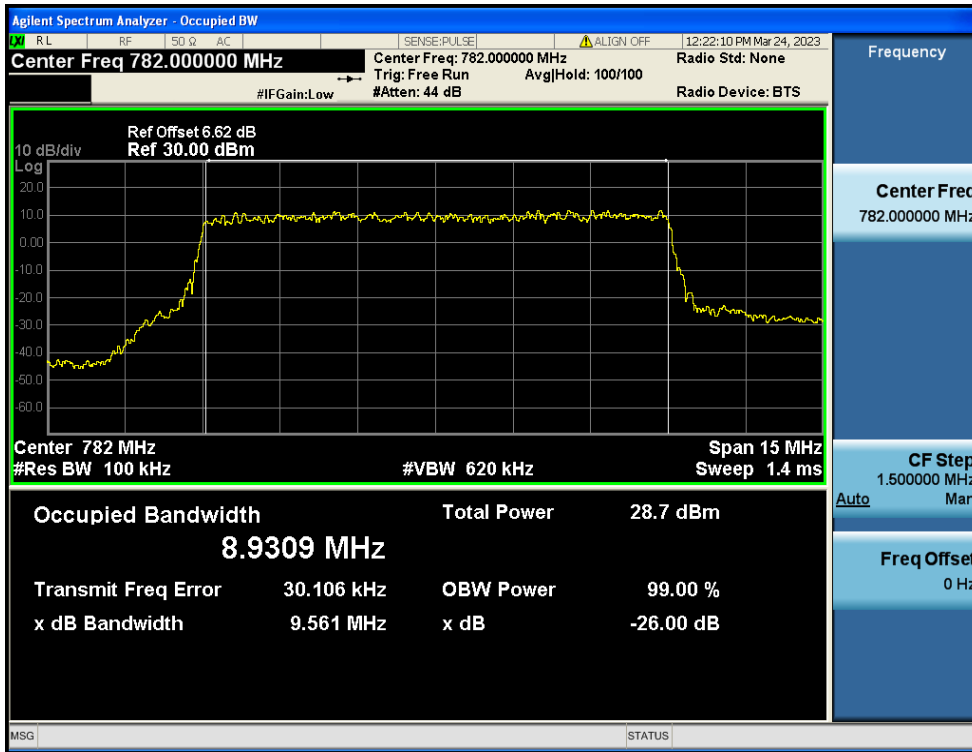
LTE Band 13 / 10MHz / QPSK - RB Size 50
