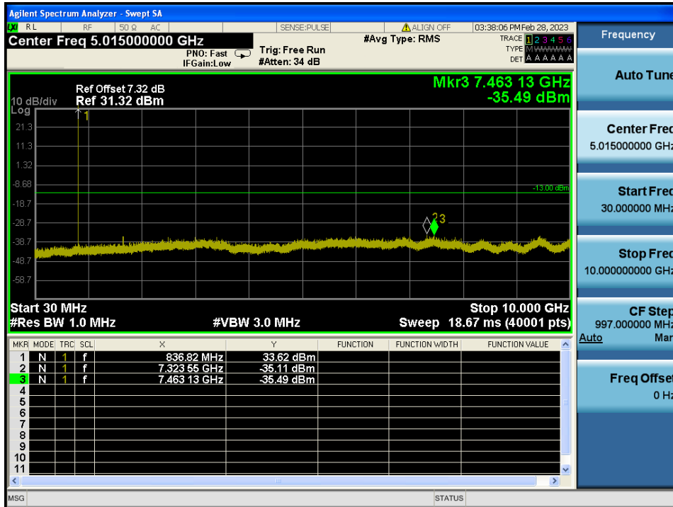
GSM850 & Channel: 190
