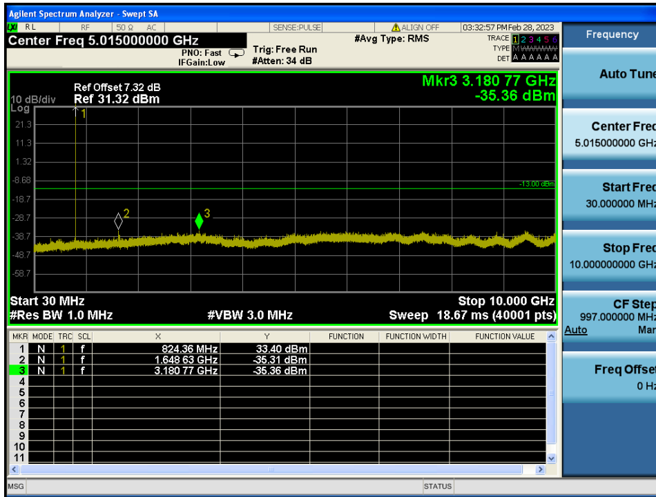
GSM850 & Channel: 128
