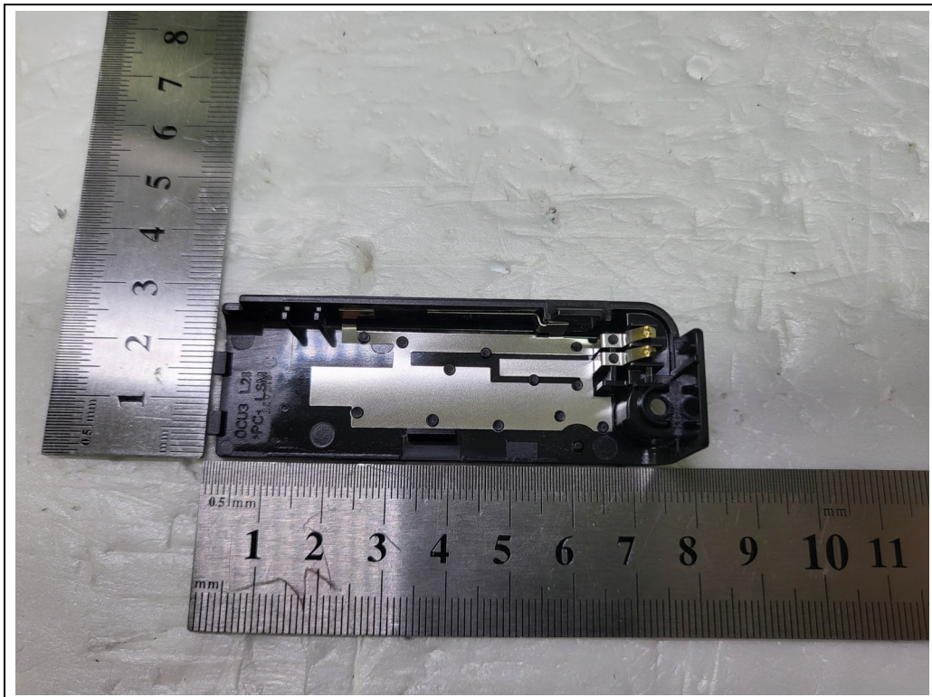
<Intenal Antenna>
