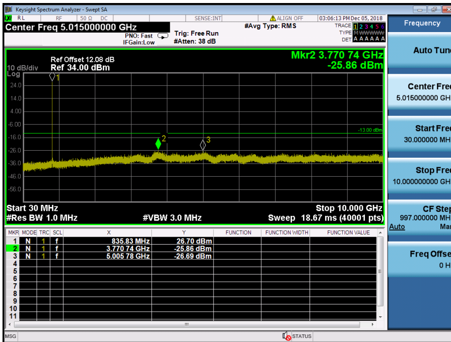
LTE Band 5 / 3MHz / QPSK - RB Size/Offset (8/0) – Mid Channel
