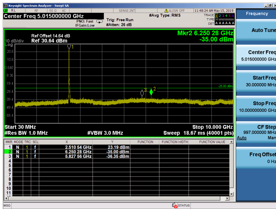
LTE Band 7 / 15MHz / QPSK - RB Size/Offset (75/0) – Low Channel
