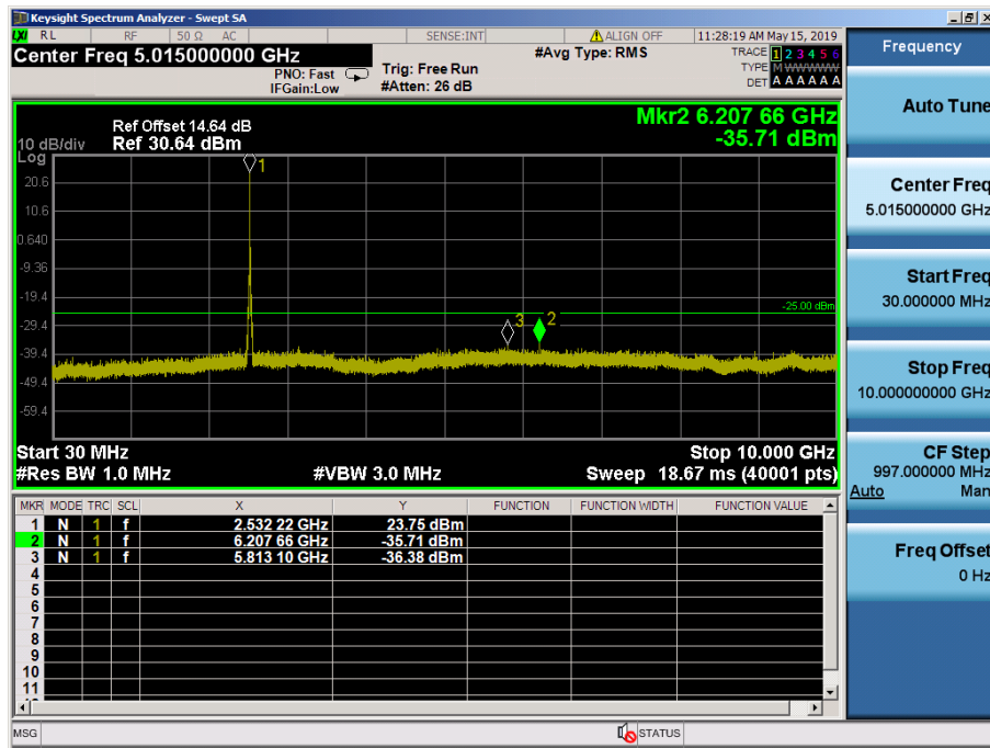
LTE Band 7 / 10MHz / QPSK - RB Size/Offset (50/0) – Mid Channel
