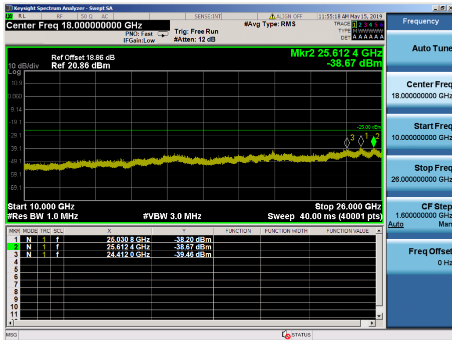
LTE Band 7 / 15MHz / QPSK - RB Size/Offset (36/18) – Mid Channel
