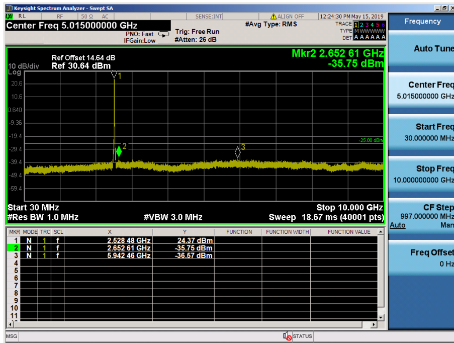
LTE Band 7 / 20MHz / QPSK - RB Size/Offset (50/0) – Mid Channel
