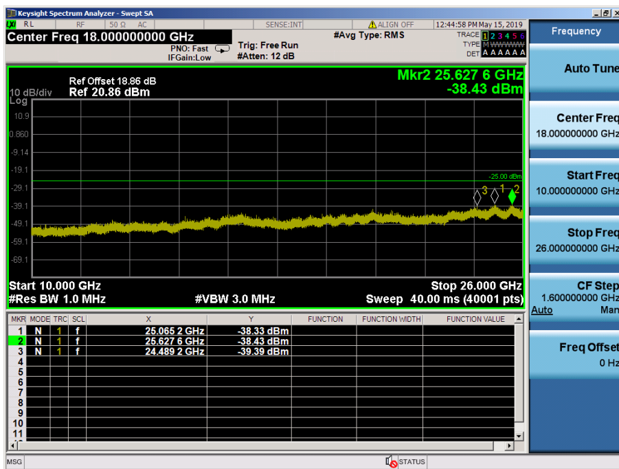
LTE Band 7 / 5MHz / 16QAM - RB Size/Offset (12/6) – Low Channel
