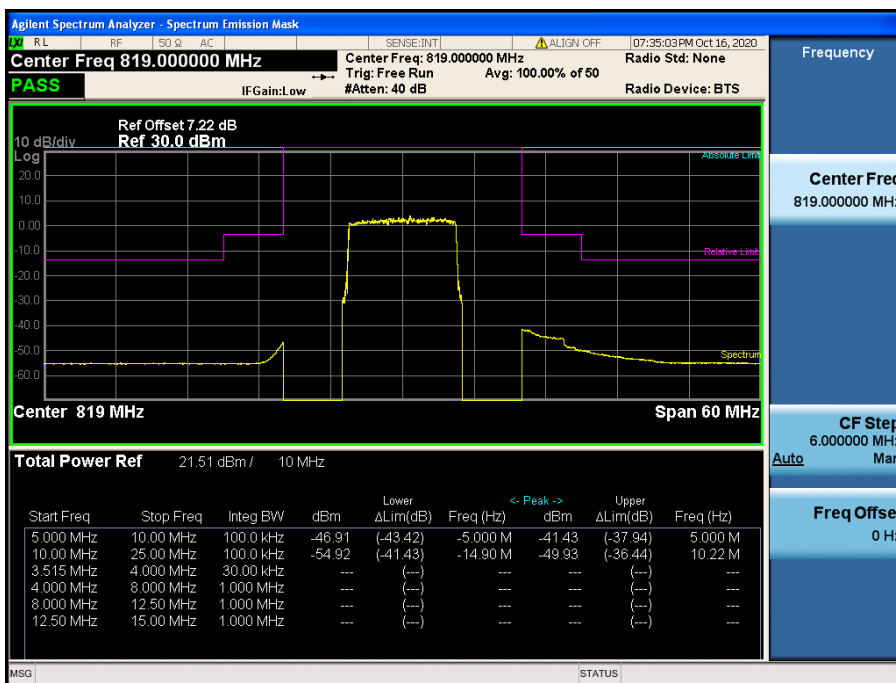
LTE Band 26 / 10 MHz / QPSK - RB Size/Offset (50/0) - Low Channel
