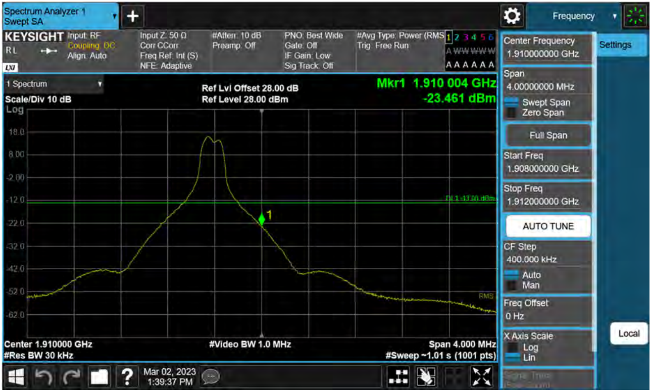
Sub6 n2. Upper Band Edge Plot (10 M BW Ch.381000 BPSK_RB1_Offset 51) -1
