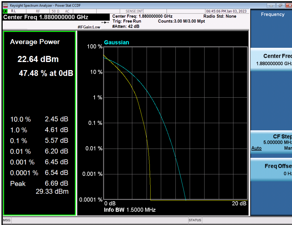
LTE Band 2 / 1.4MHz / QPSK - RB Size 6
