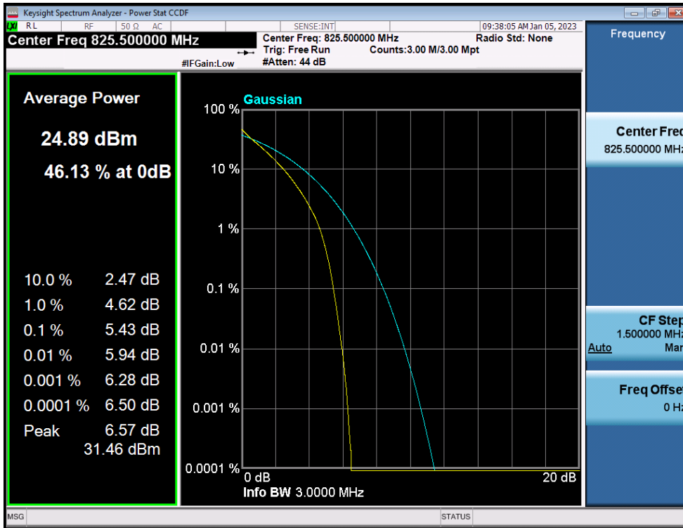
LTE Band 5 / 3MHz / QPSK - RB Size 15
