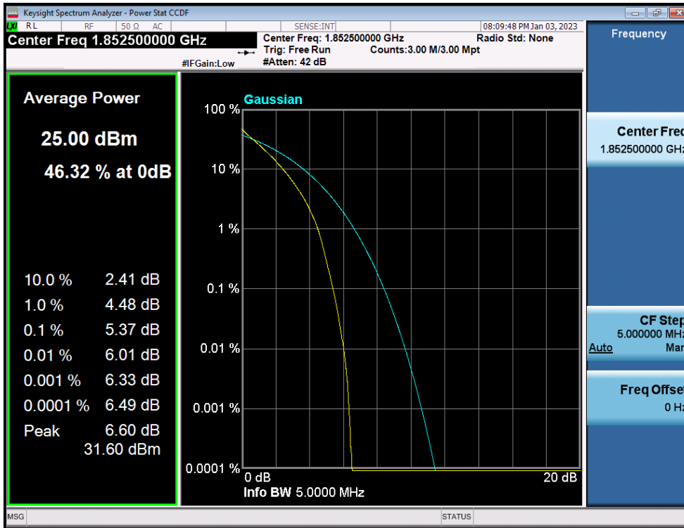
LTE Band 2 / 5MHz / QPSK - RB Size 25
