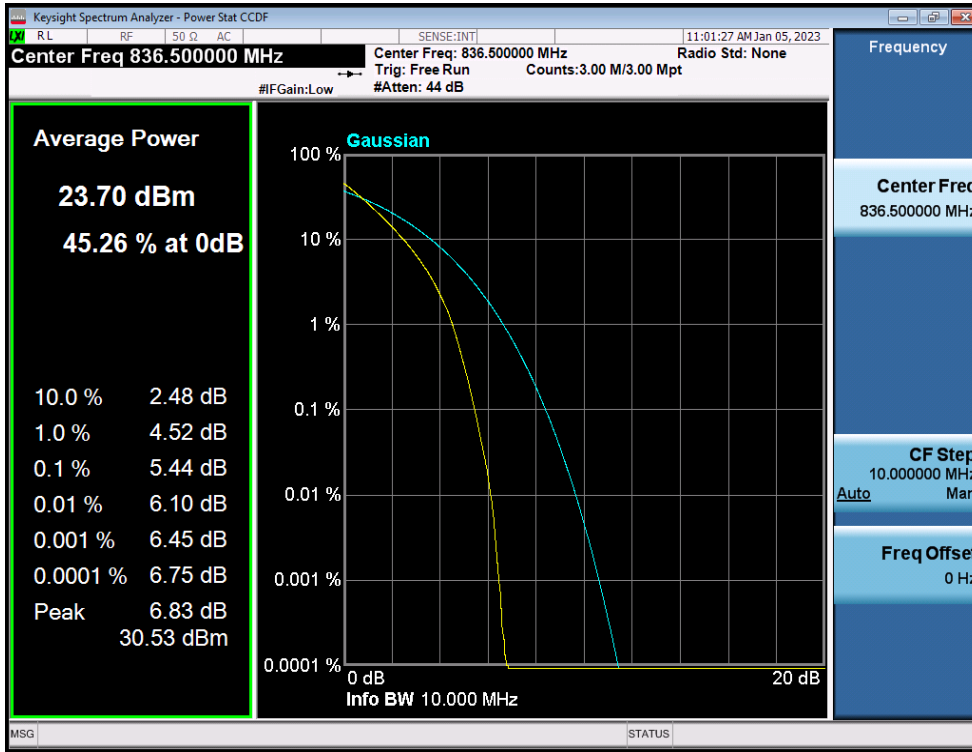
LTE Band 5 / 10MHz / QPSK - RB Size 50
