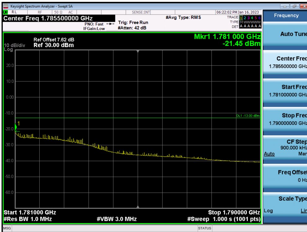
LTE Band 66(4) / 10MHz / QPSK - RB Size/Offset (25/25)
