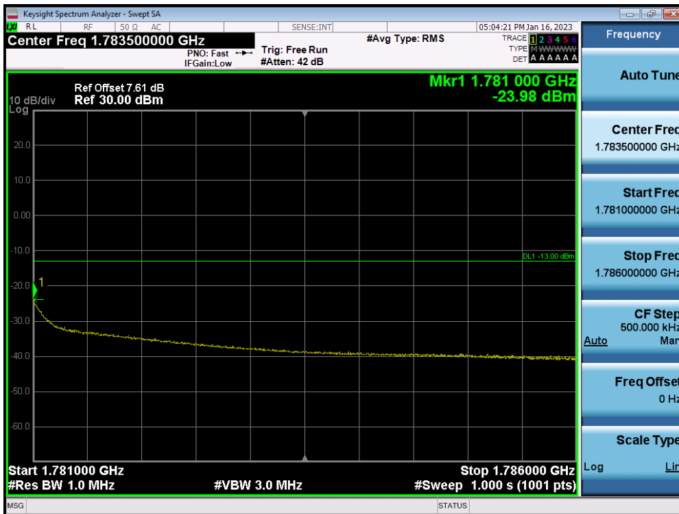
LTE Band 66(4) / 1.4MHz / QPSK - RB Size/Offset (3/0)
