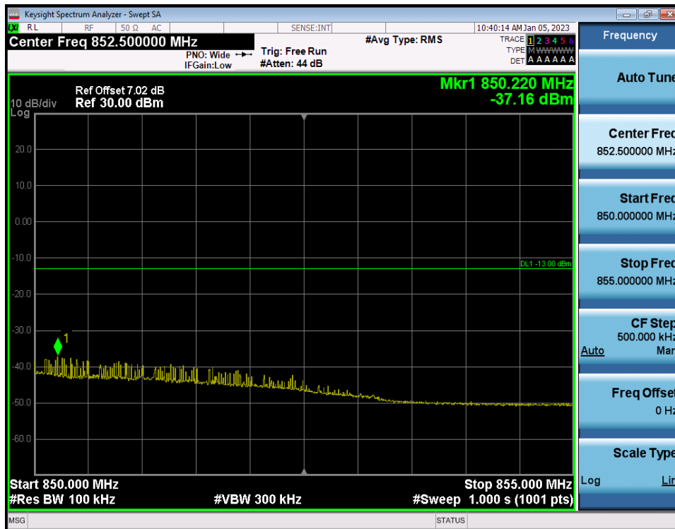
LTE Band 5 / 5MHz / QPSK - RB Size/Offset (25/0)
