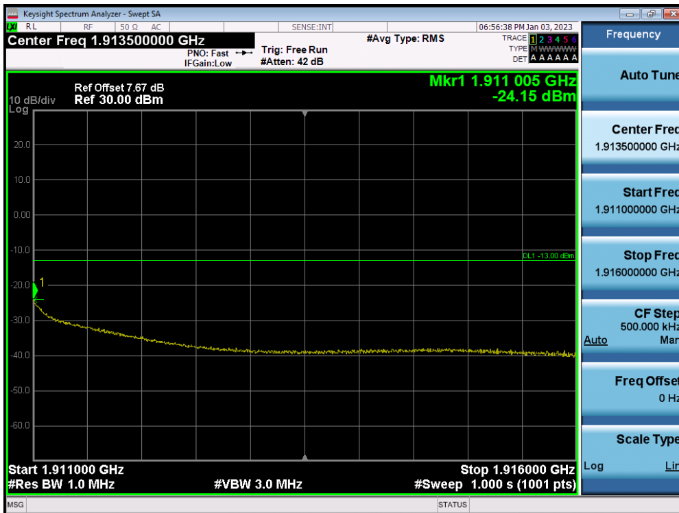
LTE Band 2 / 1.4MHz / QPSK - RB Size/Offset (3/0)
