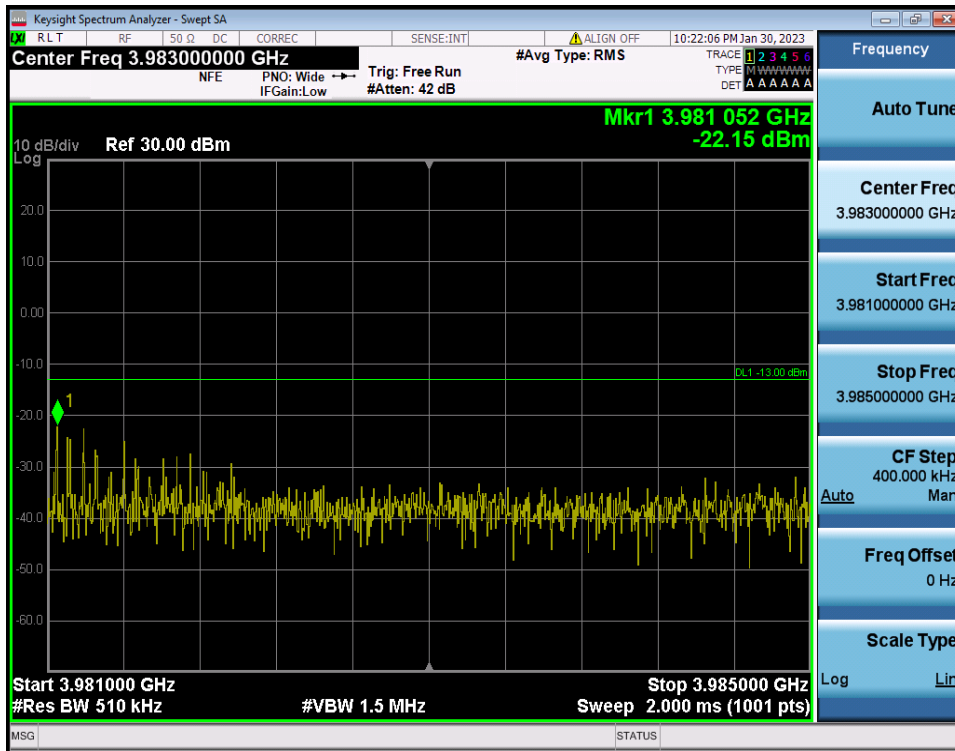
100 MHz / \pi/2 BPSK / RB Size/Offset (1RB/Inner Right)
