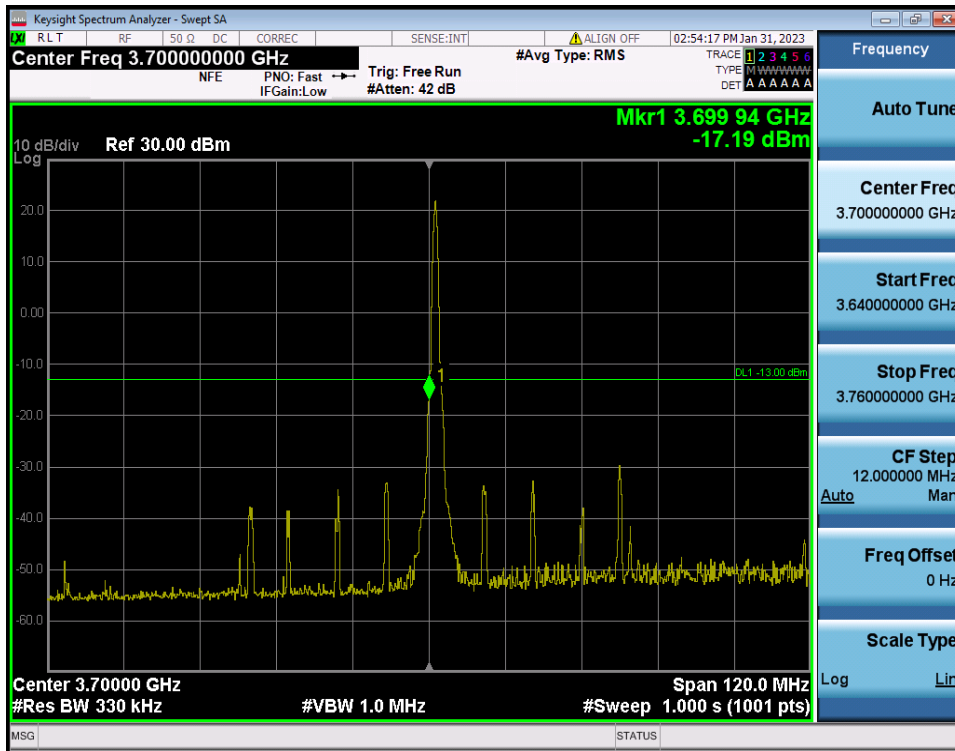
60 MHz / \pi/2 BPSK / RB Size/Offset (1RB/Edge Left)
