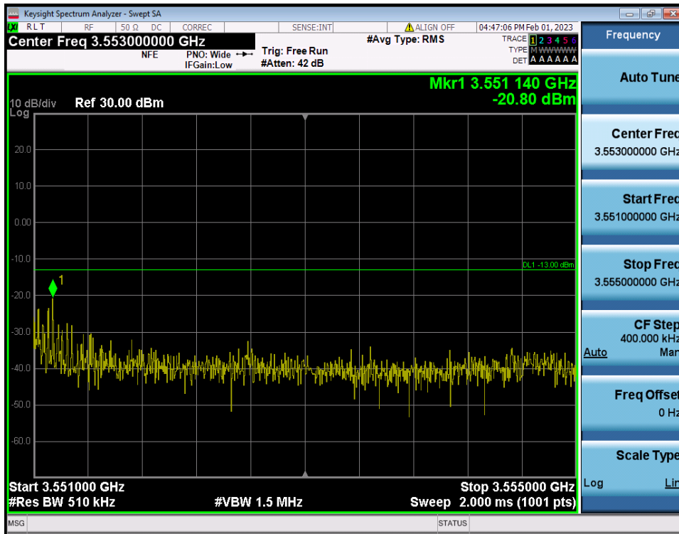
60 MHz / \pi/2 BPSK / RB Size/Offset (1RB/Inner Right)
