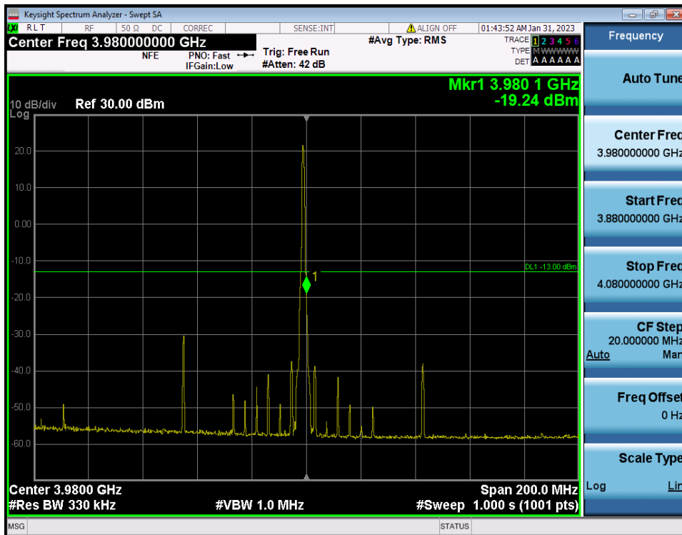
90 MHz / \pi/2 BPSK / RB Size/Offset (1RB/Edge Right)
