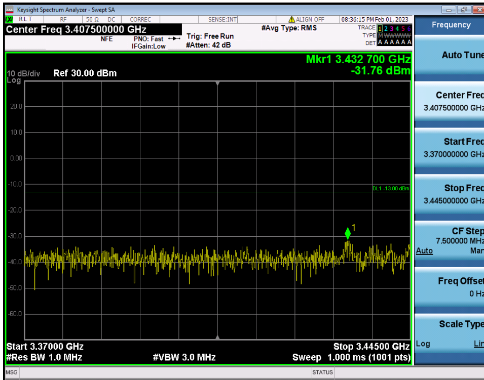
40 MHz / QPSK / RB Size/Offset (1RB/Inner Left)
