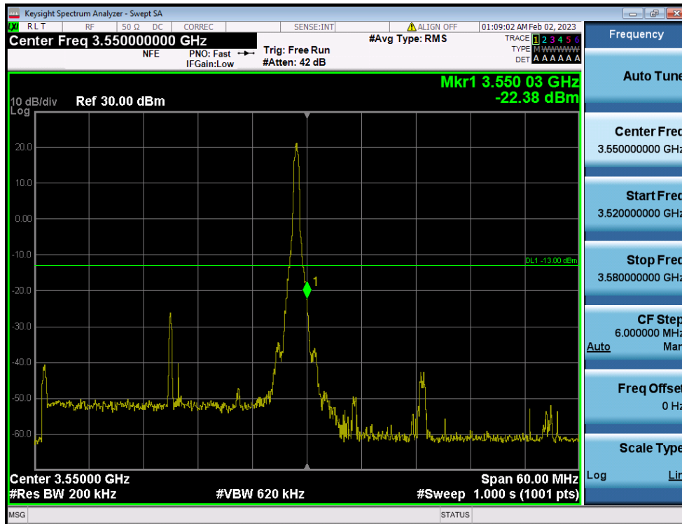
30 MHz / \pi/2 BPSK / RB Size/Offset (1RB/Edge Right)
