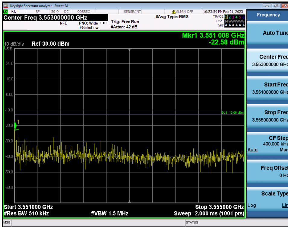
40 MHz / QPSK / RB Size/Offset (1RB/Inner Right)
