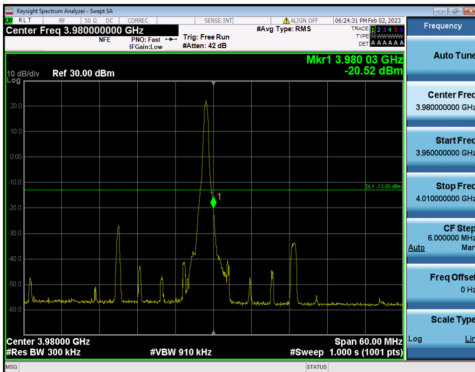
30 MHz / \pi/2 BPSK / RB Size/Offset (1RB/Edge Right)
