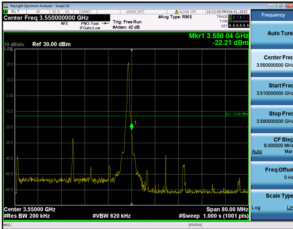
40 MHz / PI/2 BPSK / RB Size/Offset (1RB/Edge Right)
