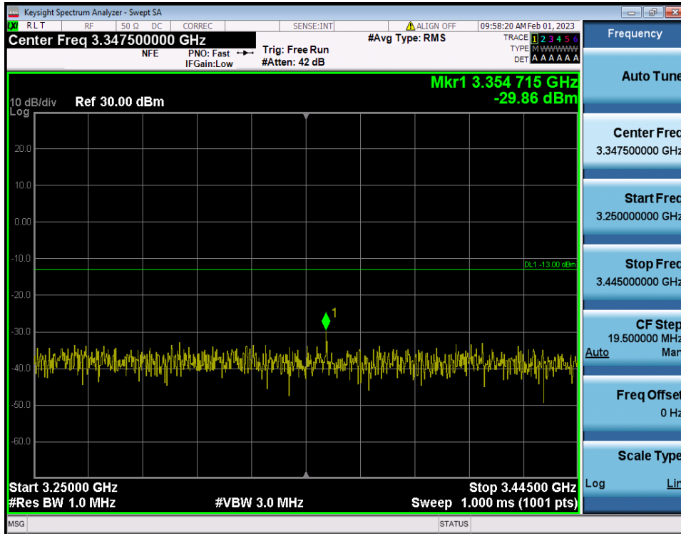
100 MHz / 16QAM / RB Size/Offset (1RB/Edge Left)
