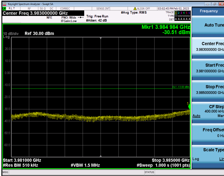
40 MHz / \pi/2 BPSK / RB Size/Offset (Full RB)
