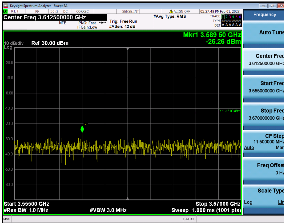
60 MHz / 256QAM / RB Size/Offset (1RB/Inner Left)
