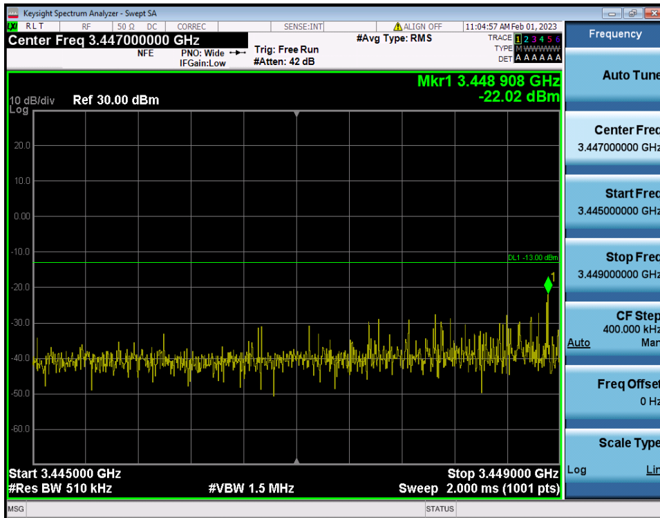
90 MHz / \pi/2 BPSK / RB Size/Offset (1RB/Inner Left)
