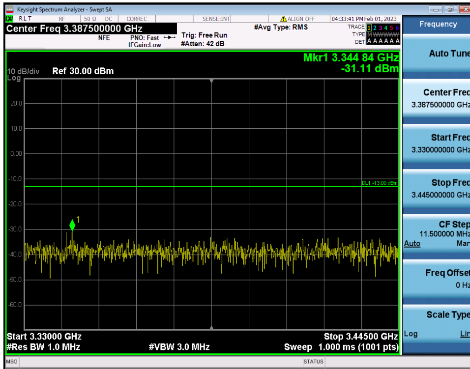
60 MHz / 256QAM / RB Size/Offset (1RB/Inner Right)
