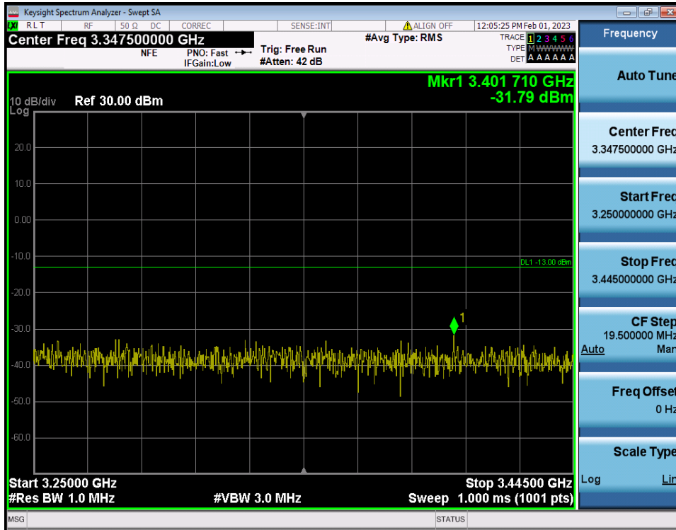
90 MHz / 256QAM / RB Size/Offset (1RB/Edge Right)
