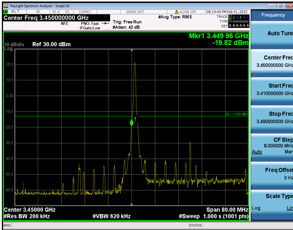
40 MHz / \pi/2 BPSK / RB Size/Offset (1RB/Edge Left)
