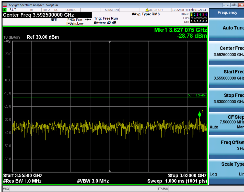
40 MHz / QPSK / RB Size/Offset (1RB/Mid)
