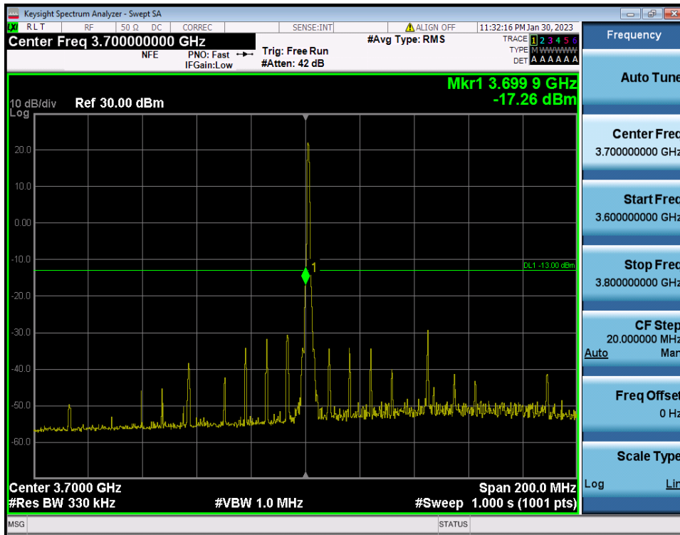
90 MHz / \pi/2 BPSK / RB Size/Offset (1RB/Edge Left)
