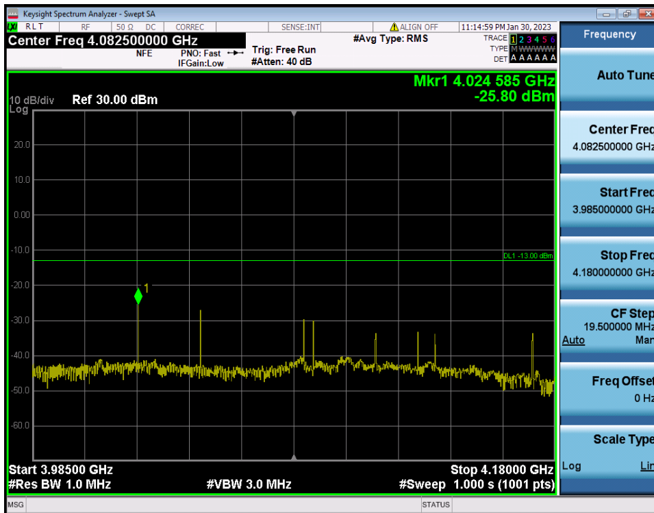
100 MHz / 256QAM / RB Size/Offset (Full RB)
