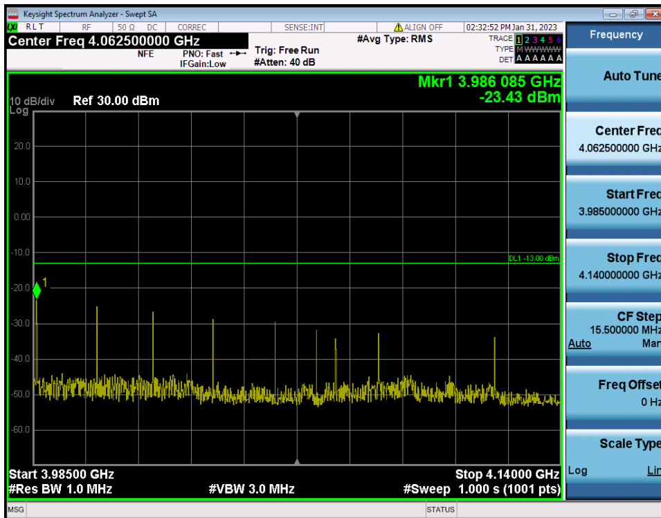
80 MHz / 256QAM / RB Size/Offset (Full RB)
