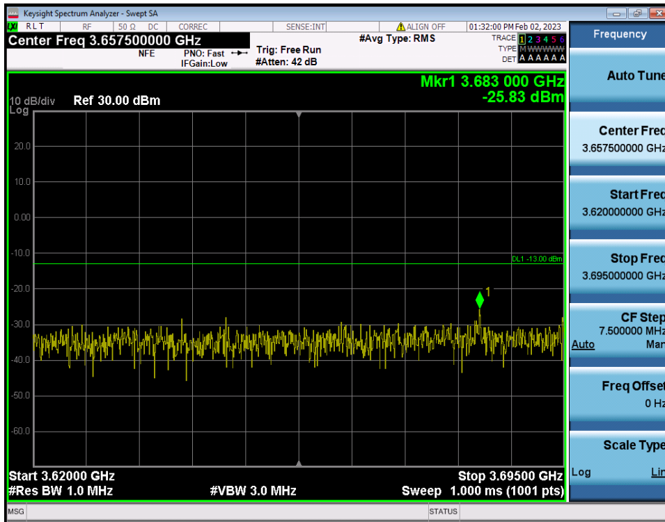
40 MHz / 16QAM / RB Size/Offset (1RB/Inner Left)
