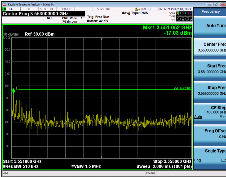
80 MHz / QPSK / RB Size/Offset (1RB/Edge Right)
