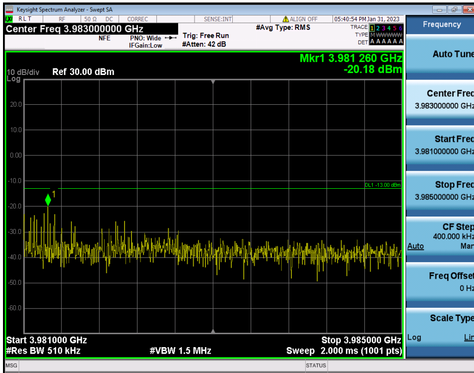
60 MHz / \pi/2 BPSK / RB Size/Offset (1RB/Edge Right)
