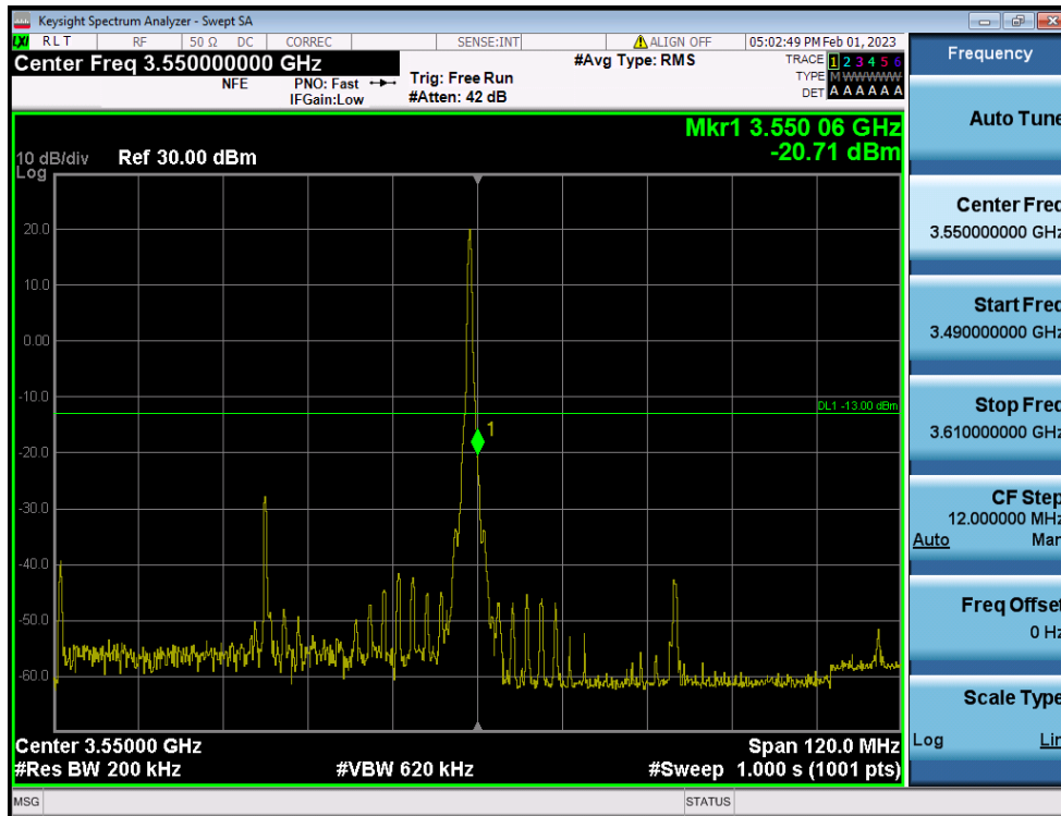
60 MHz / QPSK / RB Size/Offset (1RB/Edge Right)
