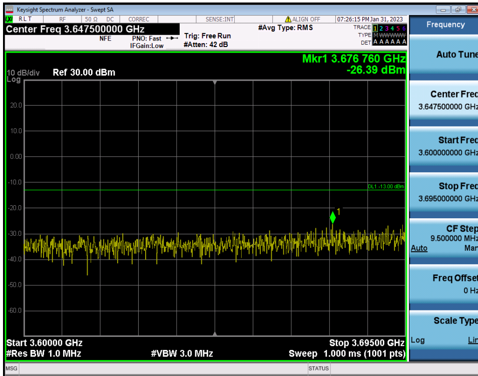
50 MHz / 64QAM / RB Size/Offset (Full RB)
