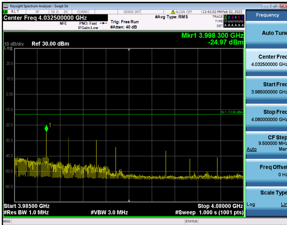
50 MHz / 256QAM / RB Size/Offset (Full RB)
