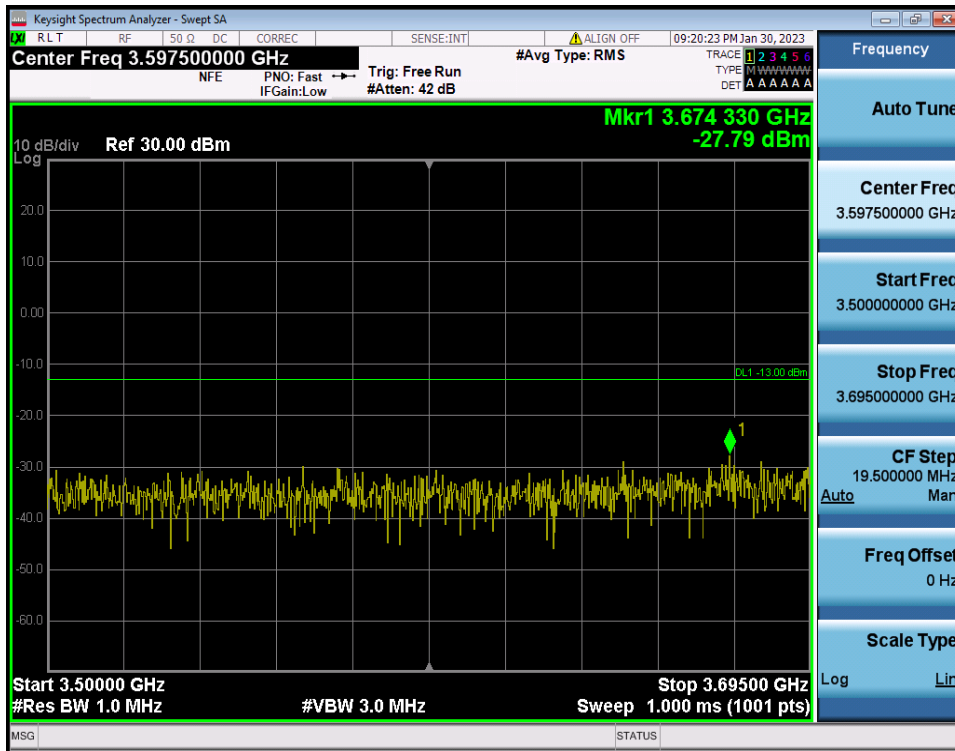
100 MHz / 256QAM / RB Size/Offset (1RB/Mid)
