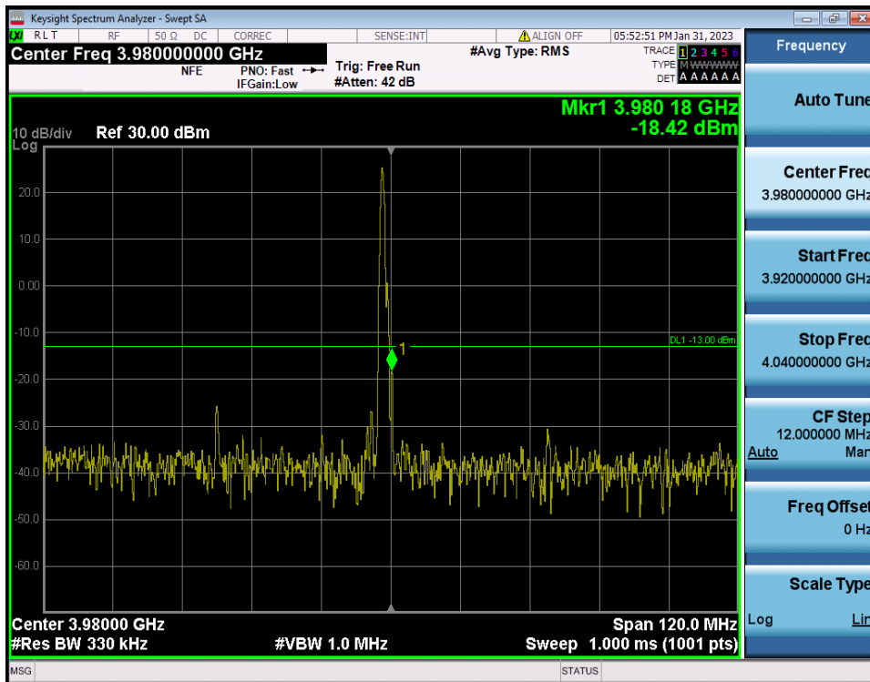
60 MHz / QPSK / RB Size/Offset (1RB/Inner Right)
