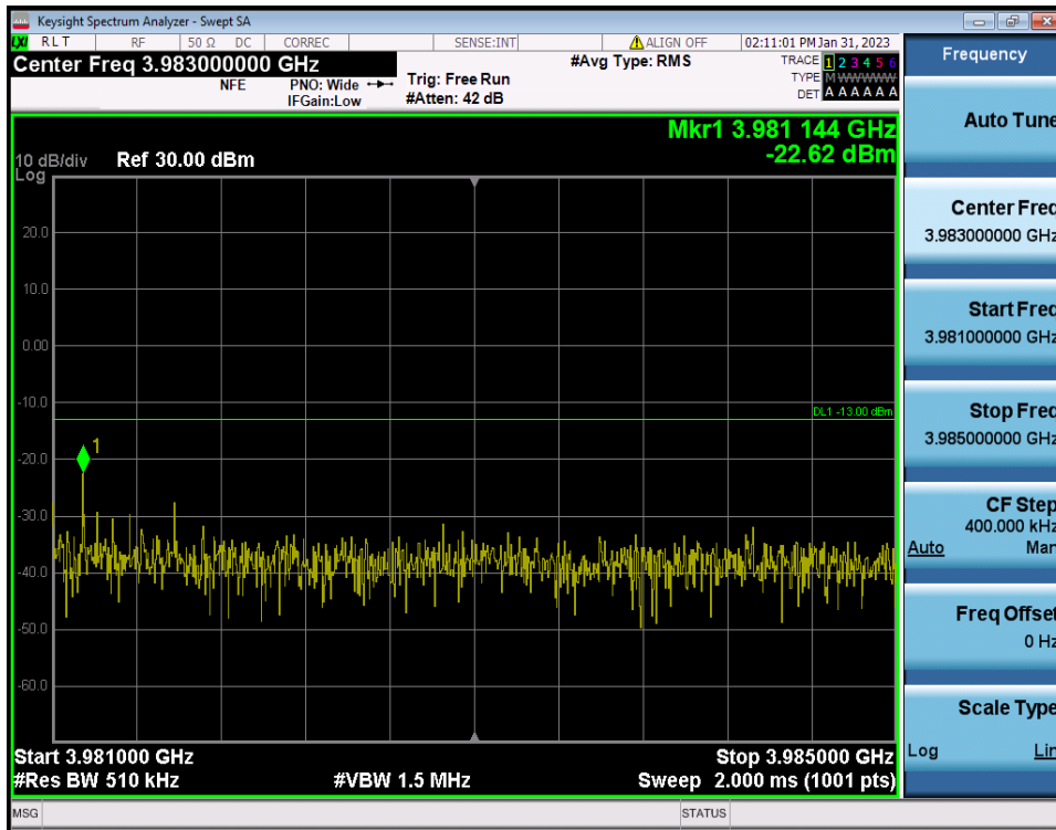
80 MHz / 16QAM / RB Size/Offset (1RB/Inner Right)
