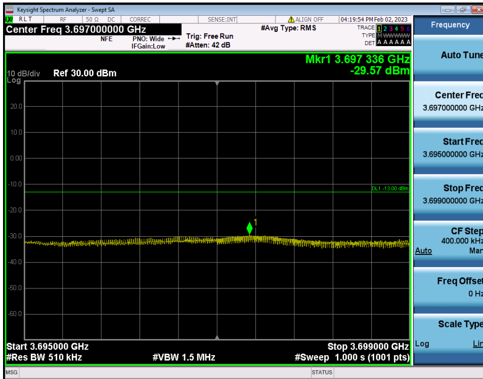
30 MHz / \pi/2 BPSK / RB Size/Offset (Full RB)
