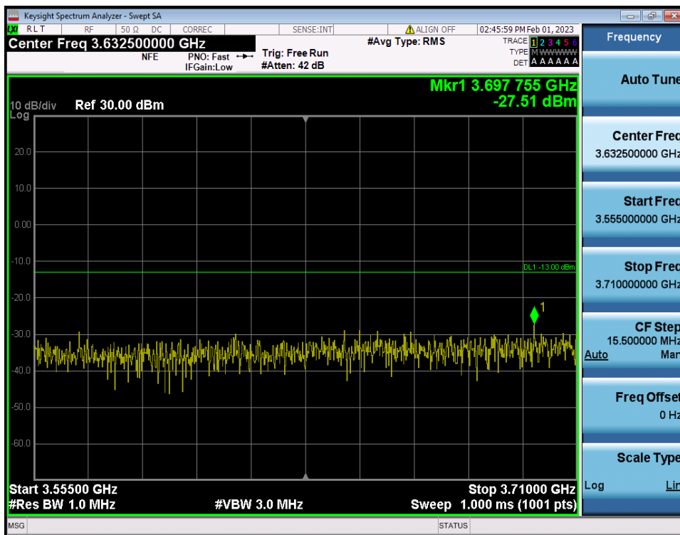
80 MHz / QPSK / RB Size/Offset (1RB/Inner Right)
