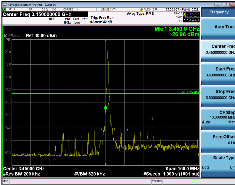
50 MHz / \pi/2 BPSK / RB Size/Offset (1RB/Edge Left)
