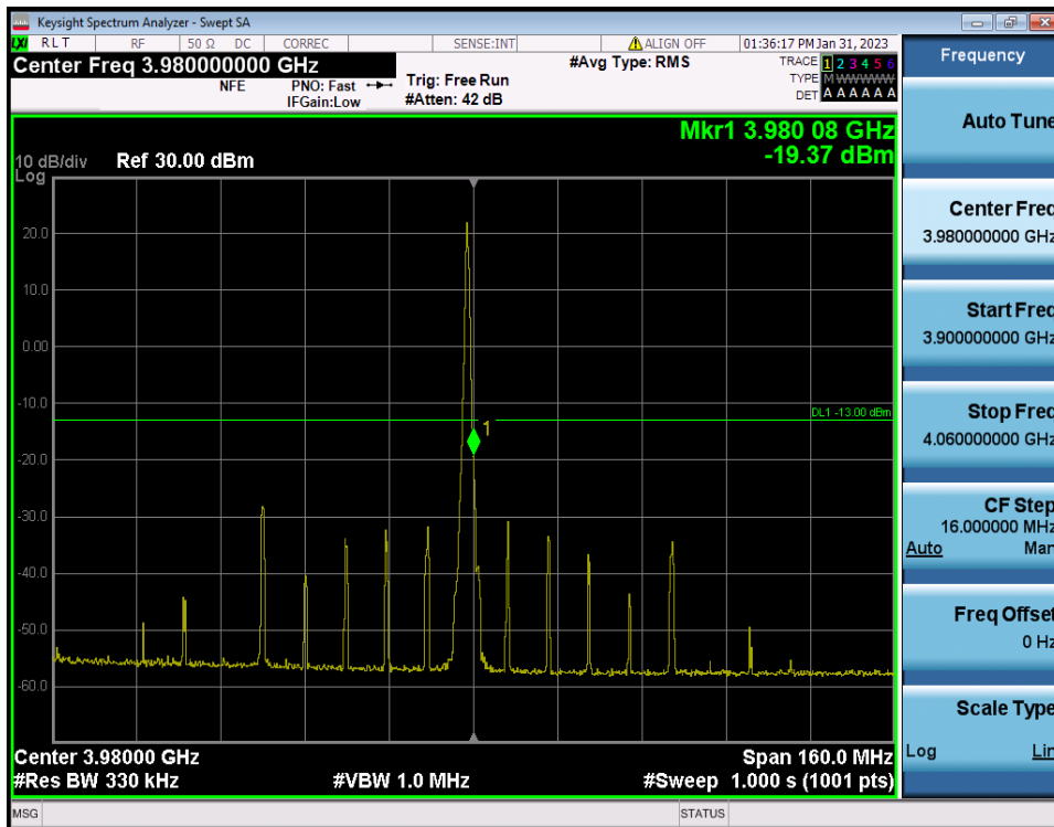
80 MHz / \pi/2 BPSK / RB Size/Offset (1RB/Edge Right)
