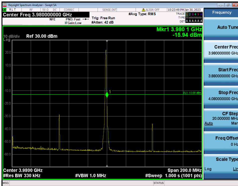
100 MHz / \pi/2 BPSK / RB Size/Offset (1RB/Edge Right)
