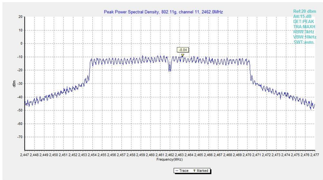
Fig.A.3.6 Power Spectral Density (802.11g, Ch 11)
