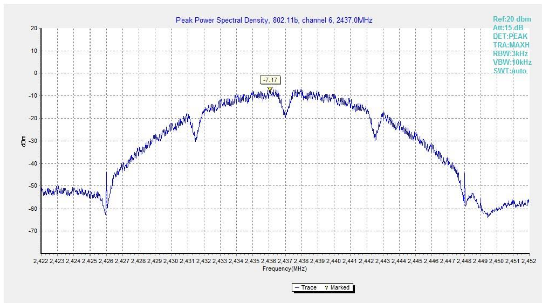
Fig.A.3.2 Power Spectral Density (802.11b, Ch 6)
