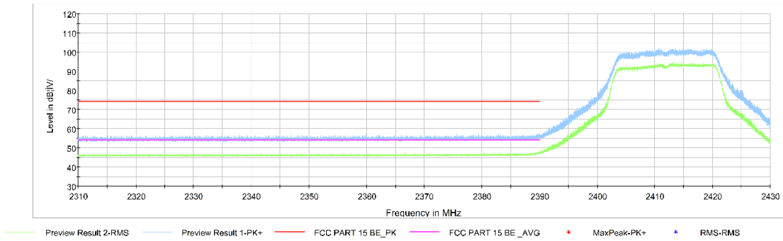
Fig.A.6.2.5 Transmitter Spurious Emission - Radiated (Power): 802.11n-HT20, ch1, 2.31 GHz - 2.43GHz
