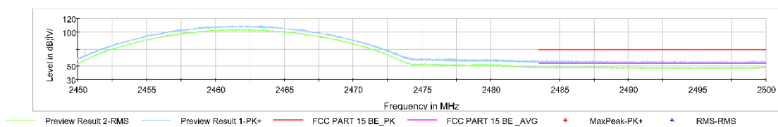
Fig.A.6.2.2 Transmitter Spurious Emission - Radiated (Power): 802.11b, ch11, 2.45 GHz - 2.50GHz
