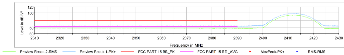
Fig.A.6.2.3 Transmitter Spurious Emission - Radiated (Power): 802.11g, ch1, 2.31 GHz - 2.43GHz
