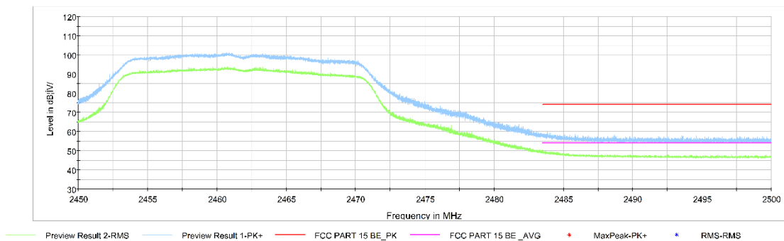
Fig.A.6.2.6 Transmitter Spurious Emission - Radiated (Power): 802.11n-HT20, ch11, 2.45 GHz - 2.50GHz
