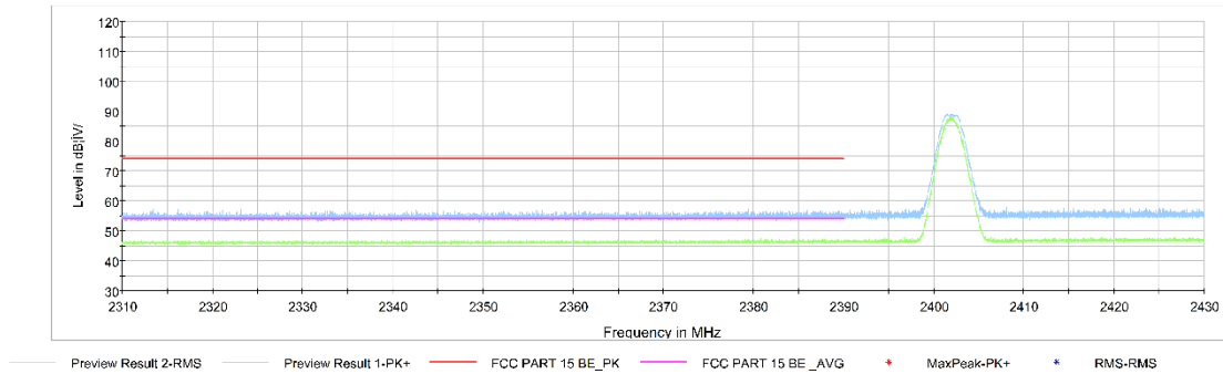
Fig.3. Frequency Band Edges: GFSK, 2402 MHz, Hopping Off, 2.31 GHz – 2.43GHz
