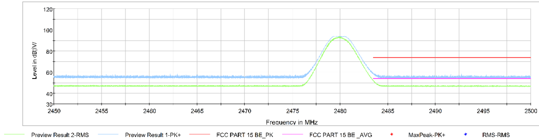
Fig.4. Frequency Band Edges: GFSK, 2480 MHz, Hopping Off , 2.45 GHz - 2.50GHz
