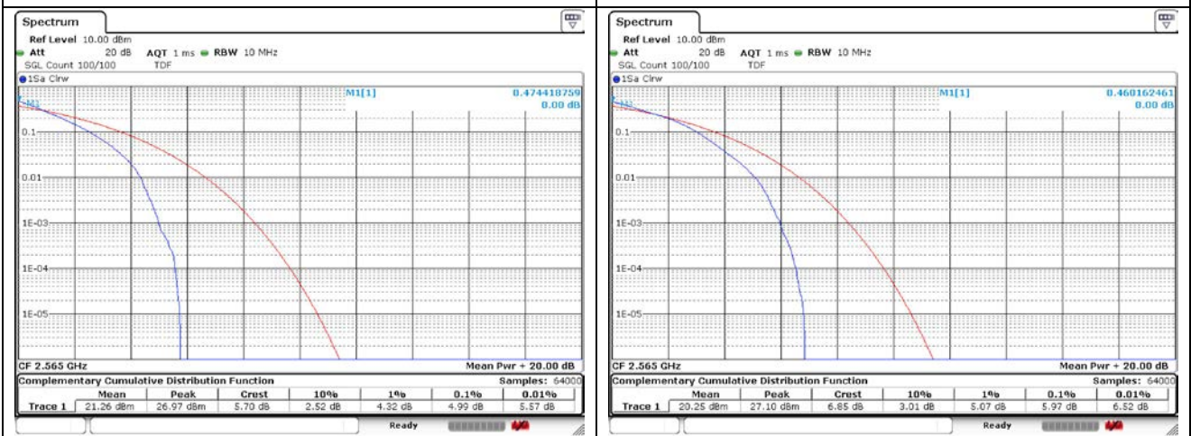
10 MHz QPSK High Channel - Full RB
