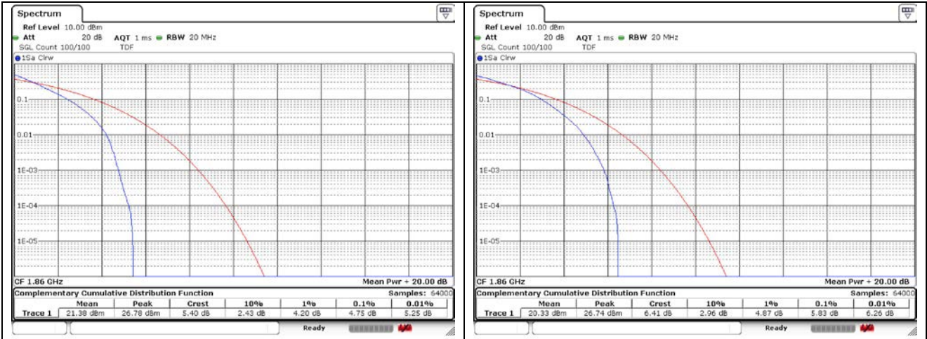
20 MHz QPSK Low Channel - Full RB
