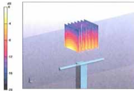
0 dB = 12.4mW/g
