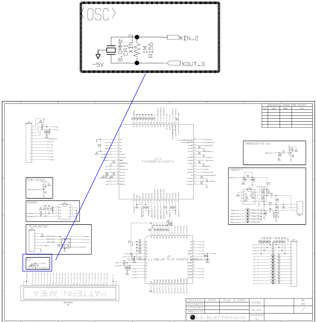
<Fig. 4. PCB Circuit Diagram>
