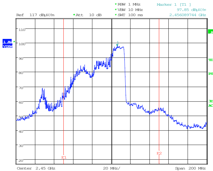
< Fig 8. Frequency Measurements (Minimum Frequency Observed: 2.456 GHz) >
