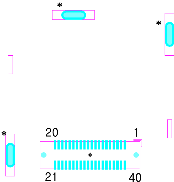
< Opposite (Host) Pin Map (Top View) >
