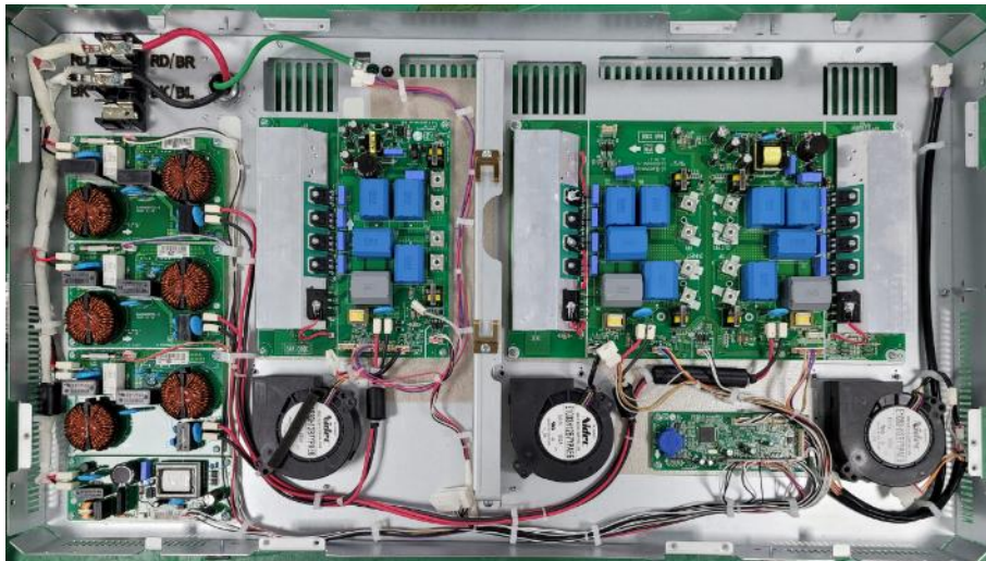
< Bottom plate >
