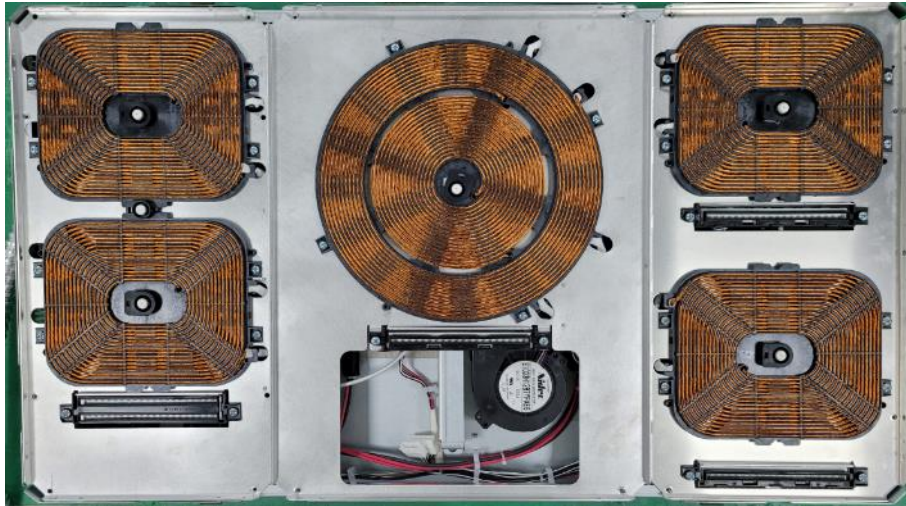
< IH core plate >
