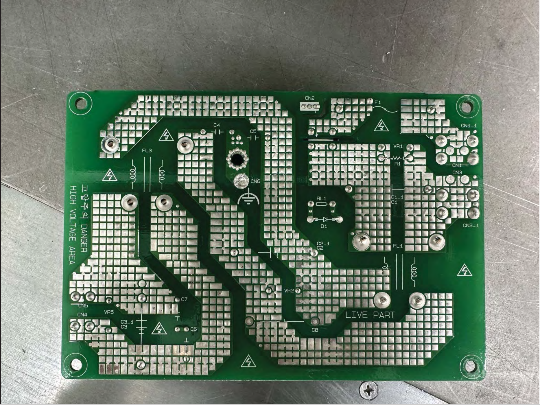
Rear View of Noise Filter PCB
