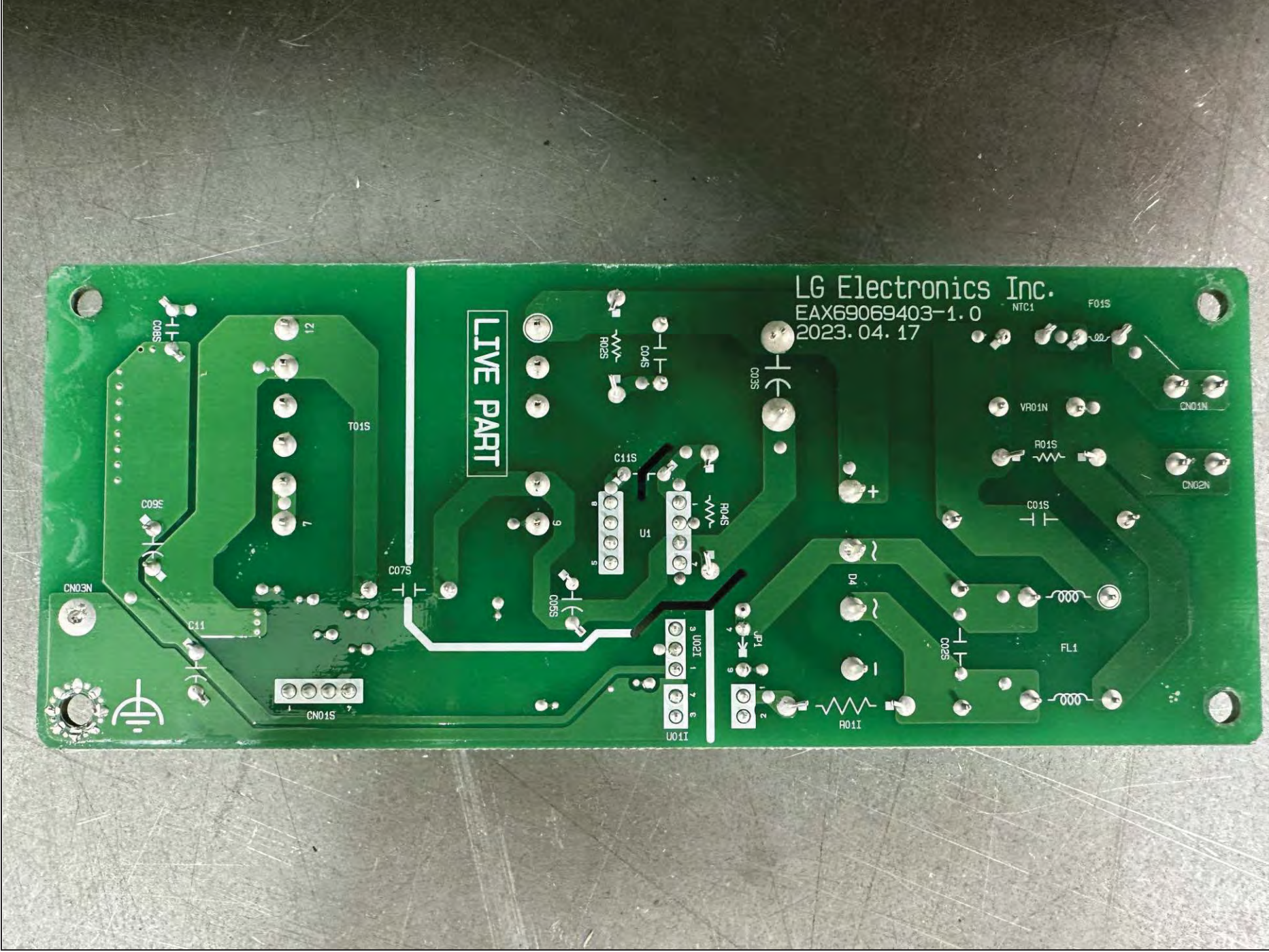
Rear View of Power SMPS
