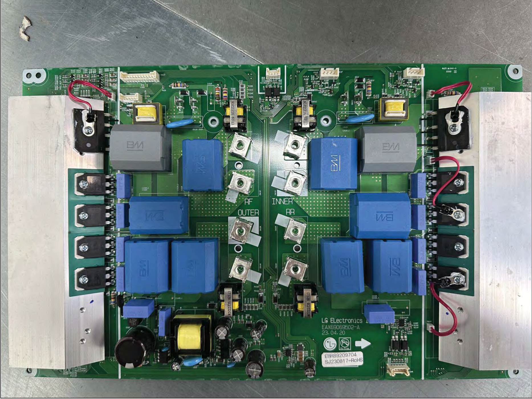
Front View of Inverter 4B PCB
