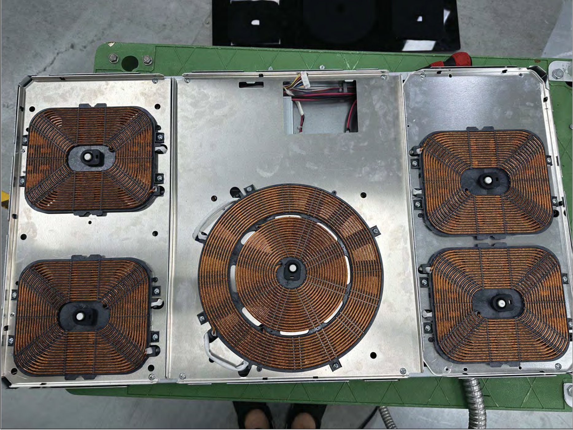
Inside(1) of EUT
