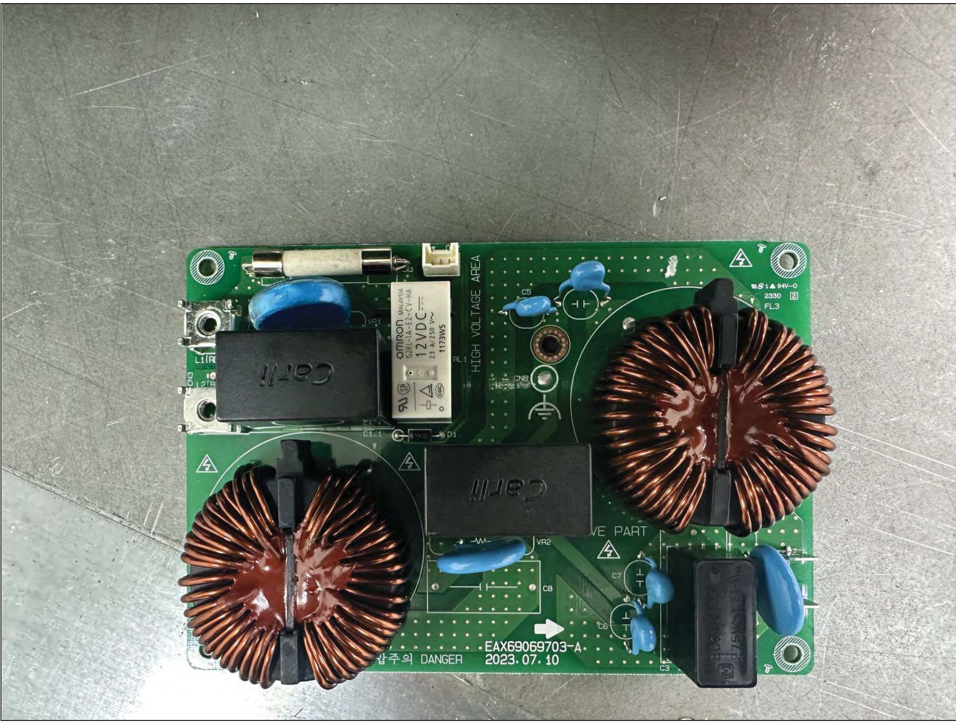
Front View of Noise Filter PCB
