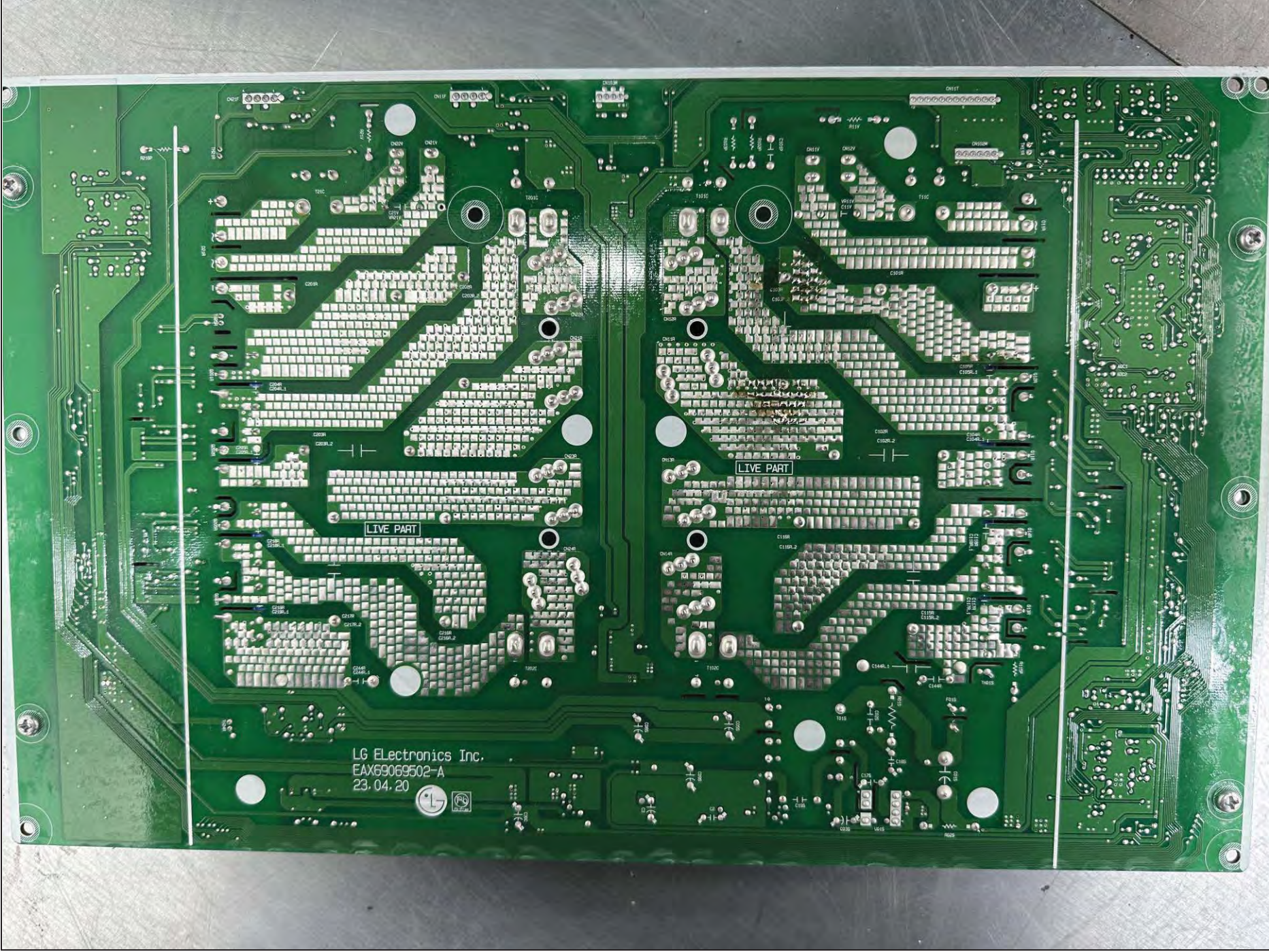
Rear View of Inverter 4B PCB
