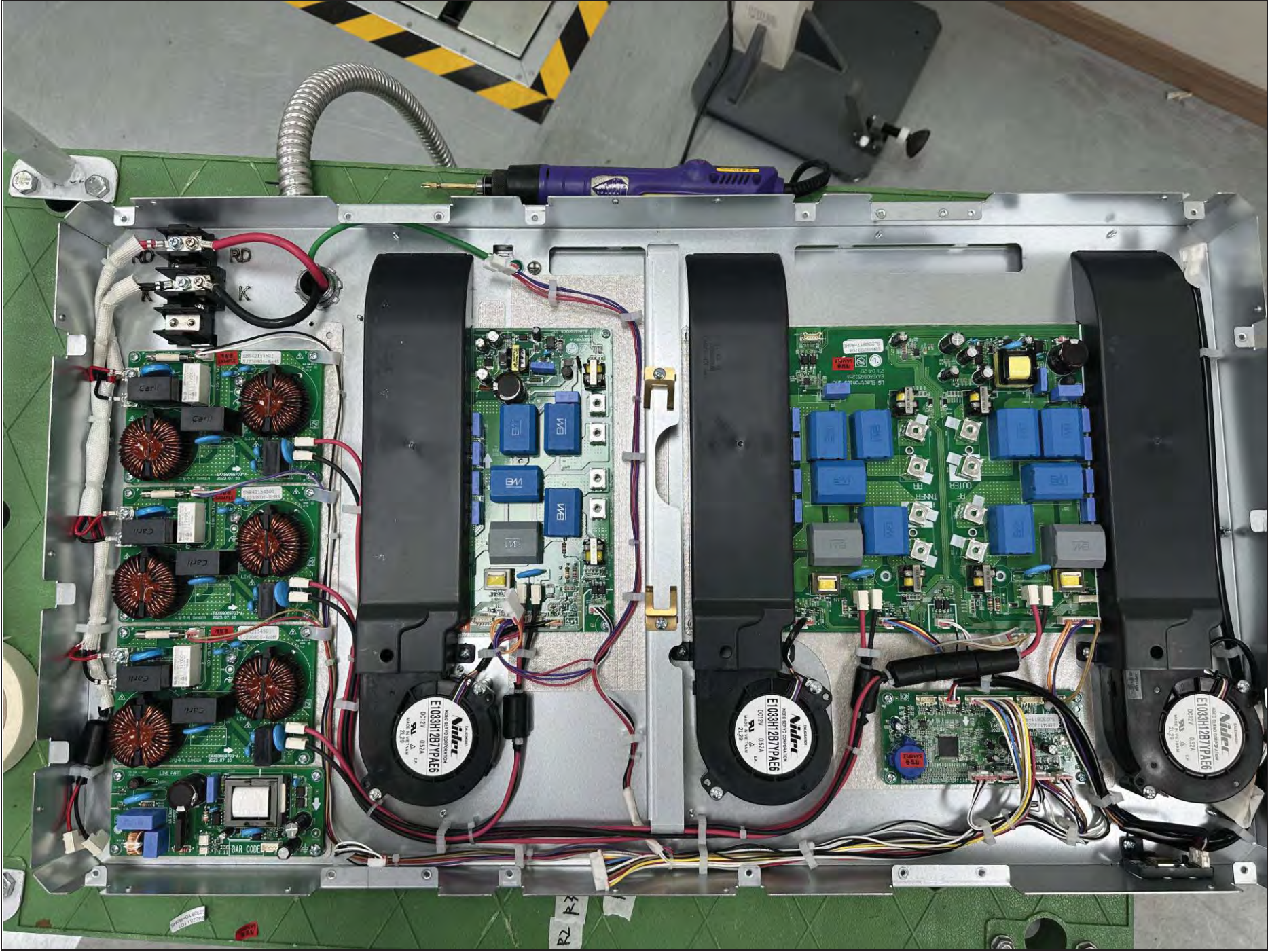
Inside(2) of EUT
