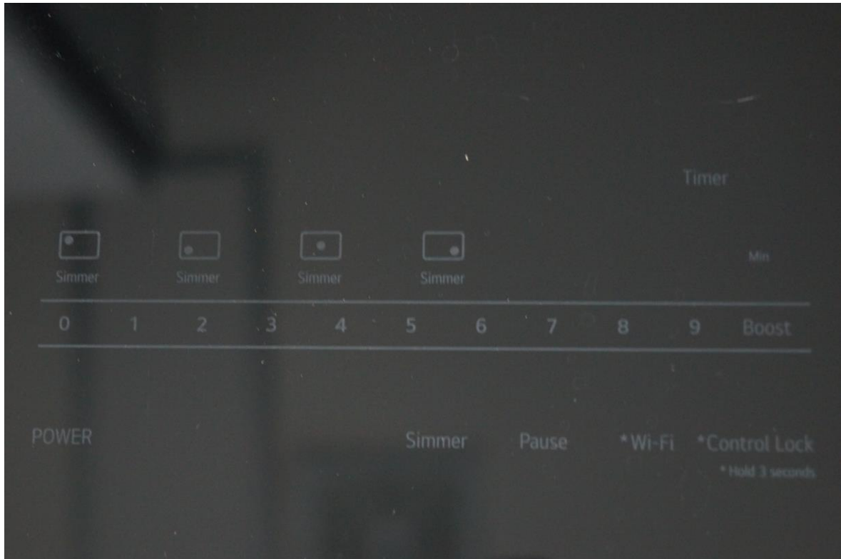
<Function key>
