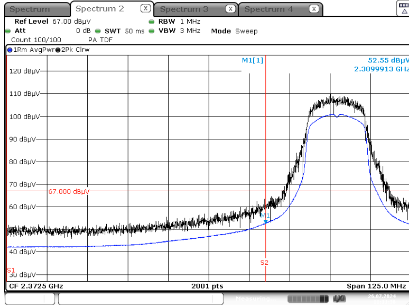
Radiated Restricted Band Edges plot - Average Reading (802.11n(HT20), Ch. 1, X-H)
