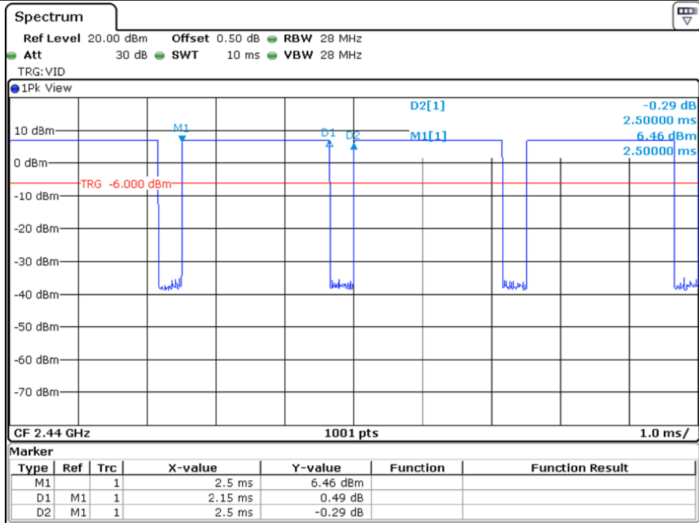
Bluetooth LE_ Packet Length: 37 Byte
