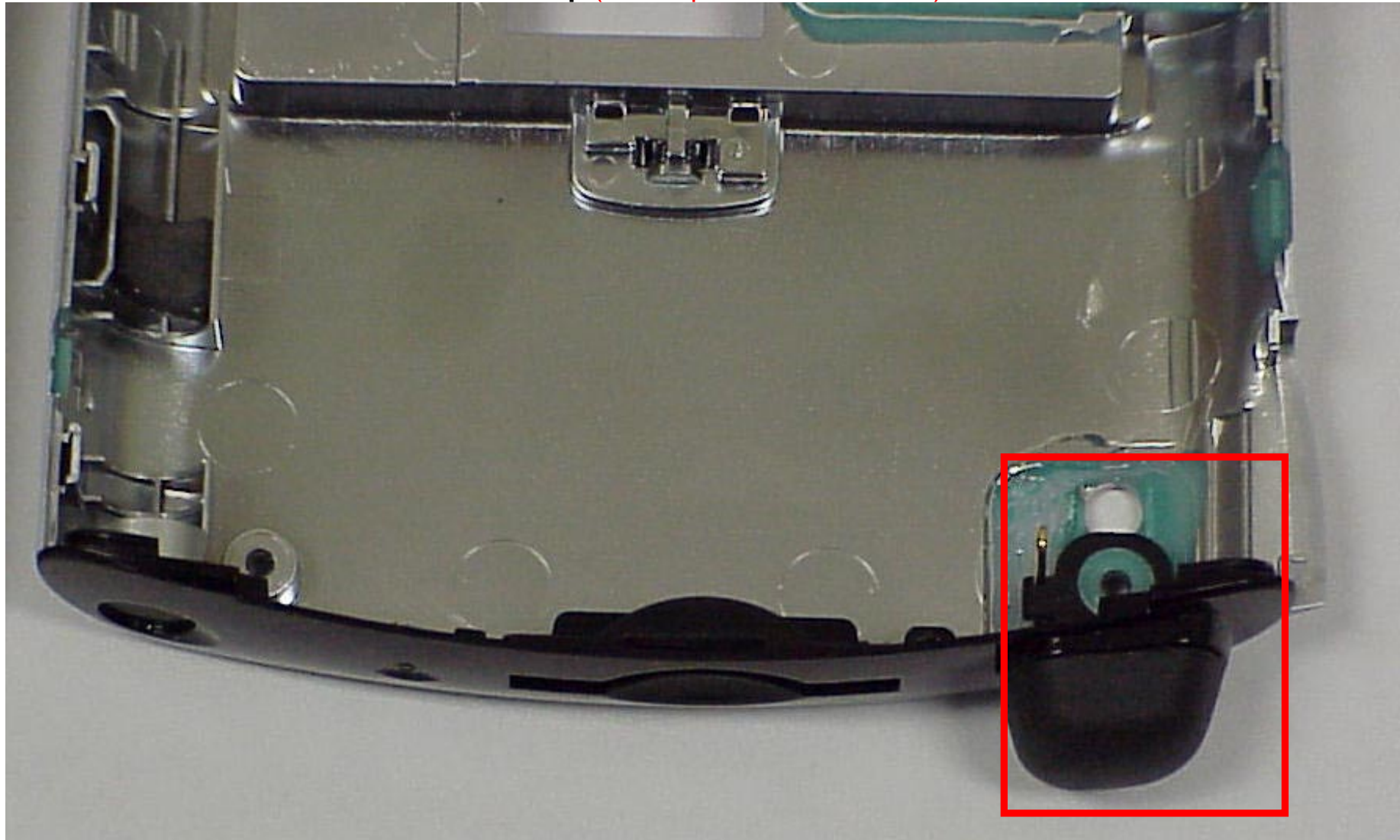
W-LAN Antenna Position Close-up (in red: position of antenna)
