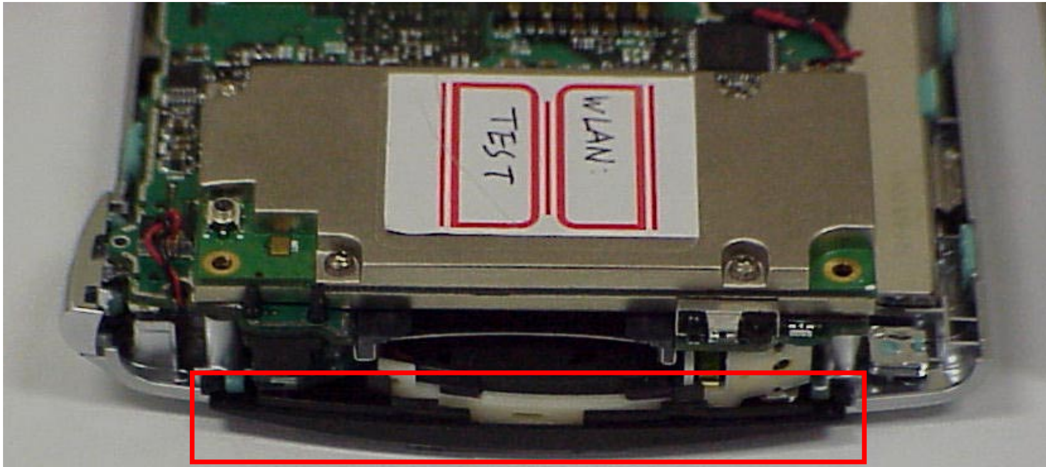
Bluetooth™ Antenna Position Close-up (in red: position of antenna)
