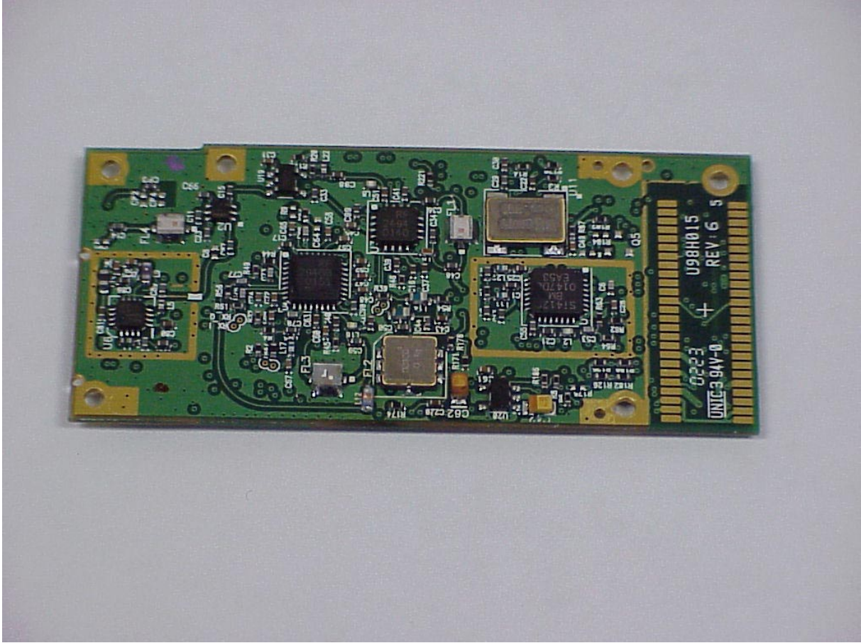
W-LAN Bottom
