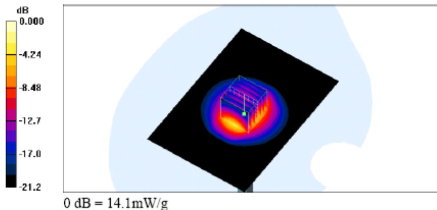
Body-Tissue-Simulating-Liquid 2.4GHz
