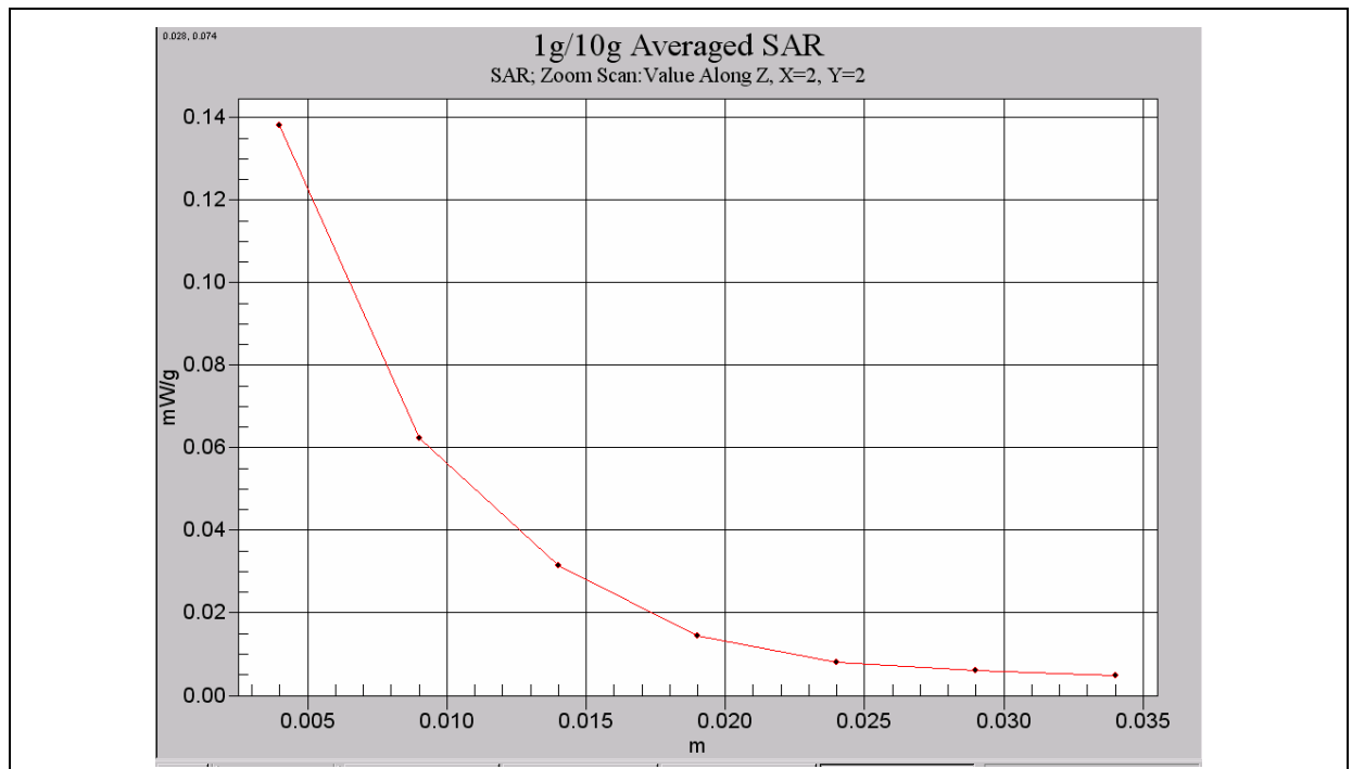
802.11b Wi-Fi Body- Channel 6 (Bluetooth on)
