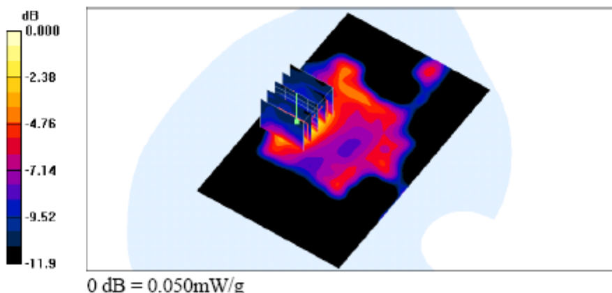
802.11g Body-SAR Test Result for Flat Position – Channel 6
