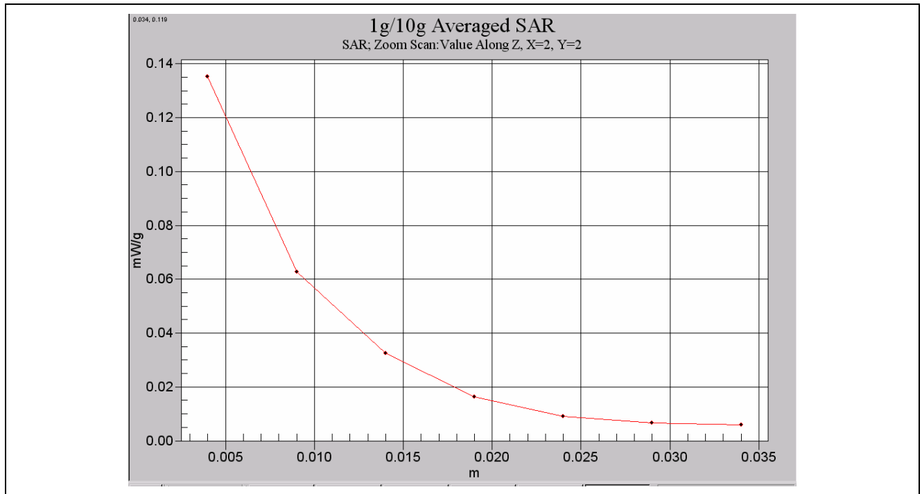
802.11b Wi-Fi Body- Channel 6 (Bluetooth off)
