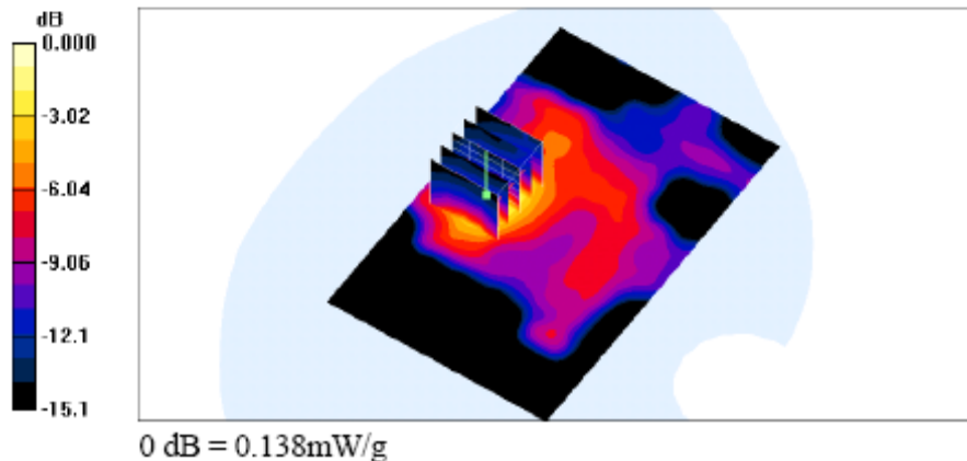
802.11b Body-SAR Test Result for Flat Position – Channel 6
