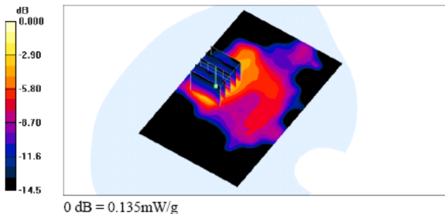
802.11b Body-SAR Test Result for Flat Position – Channel 1
