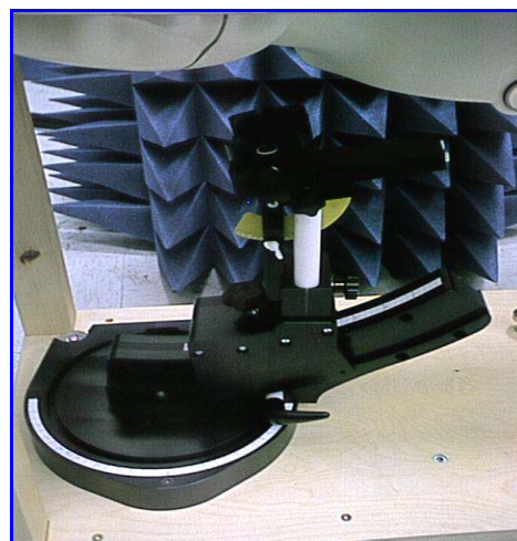
Figure 5. Device Holder
