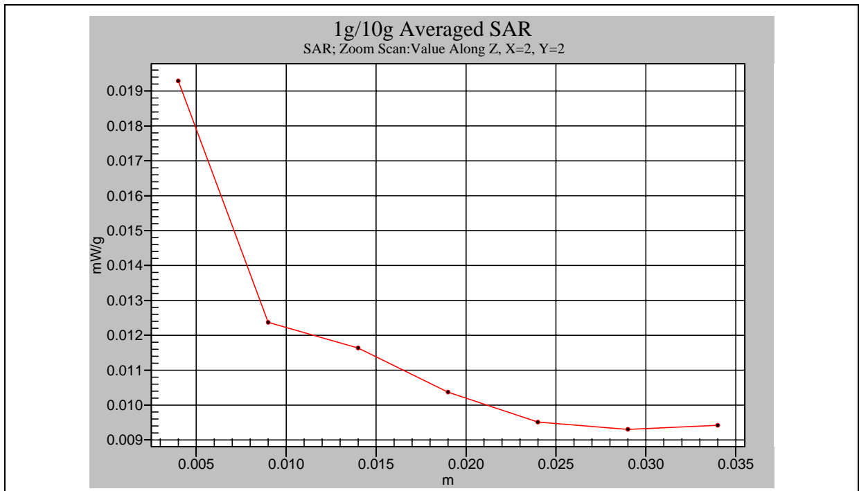
802.11g Wi-Fi Body- Channel 6 (Bluetooth off)
