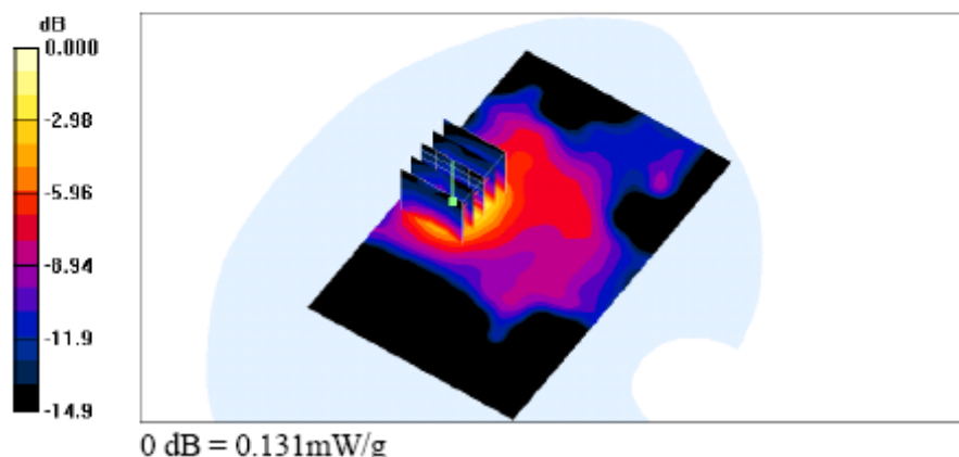
802.11b Body-SAR Test Result for Flat Position – Channel 11
