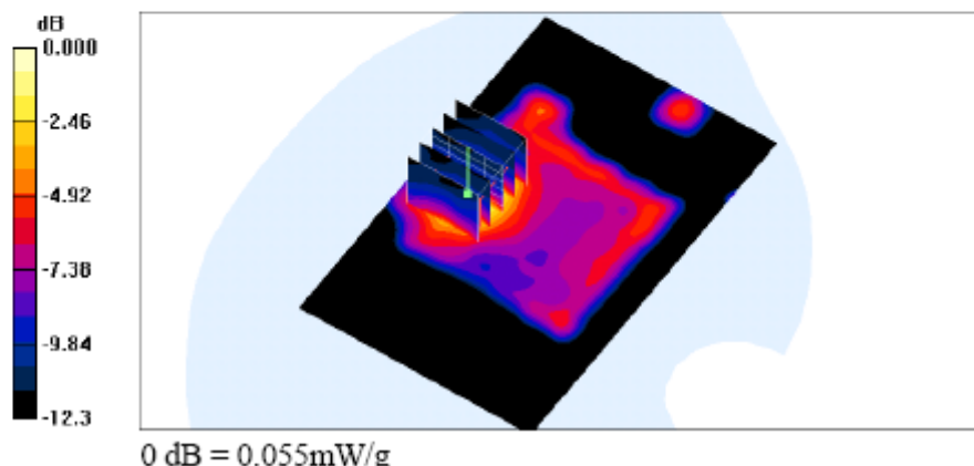
802.11g Body-SAR Test Result for Flat Position – Channel 11
