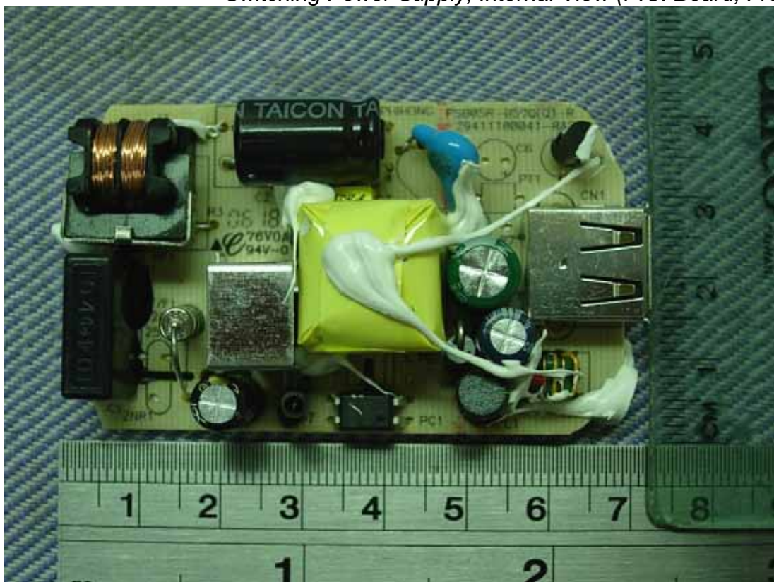
Figure 24 Switching Power Supply, Internal View (P.C. Board, Front View)
