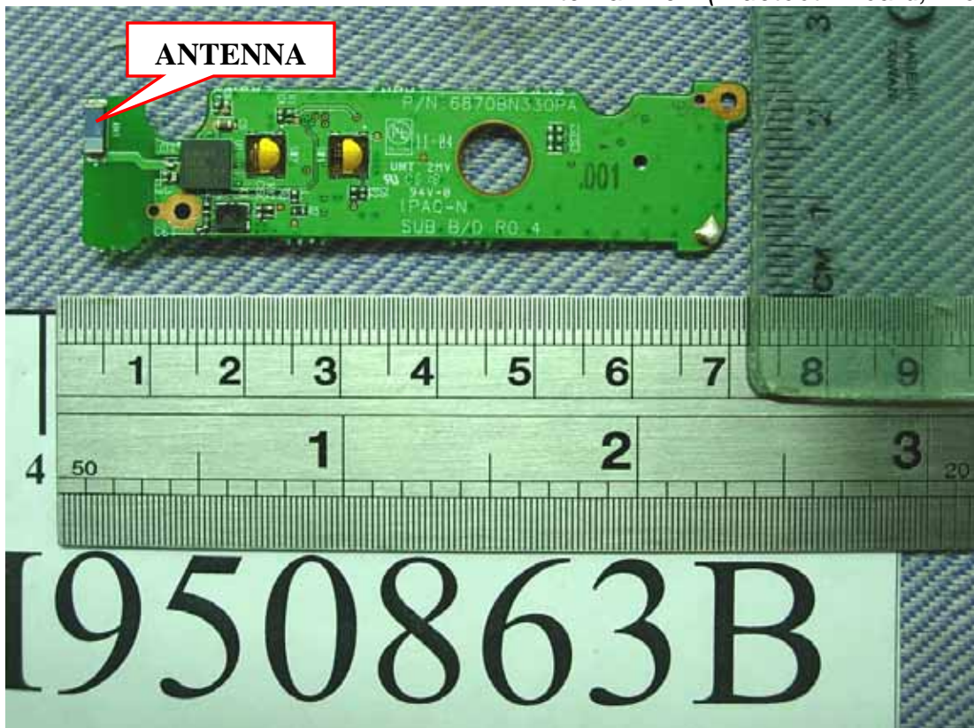
Figure 20 Internal View (Bluetooth Board, Front View)
