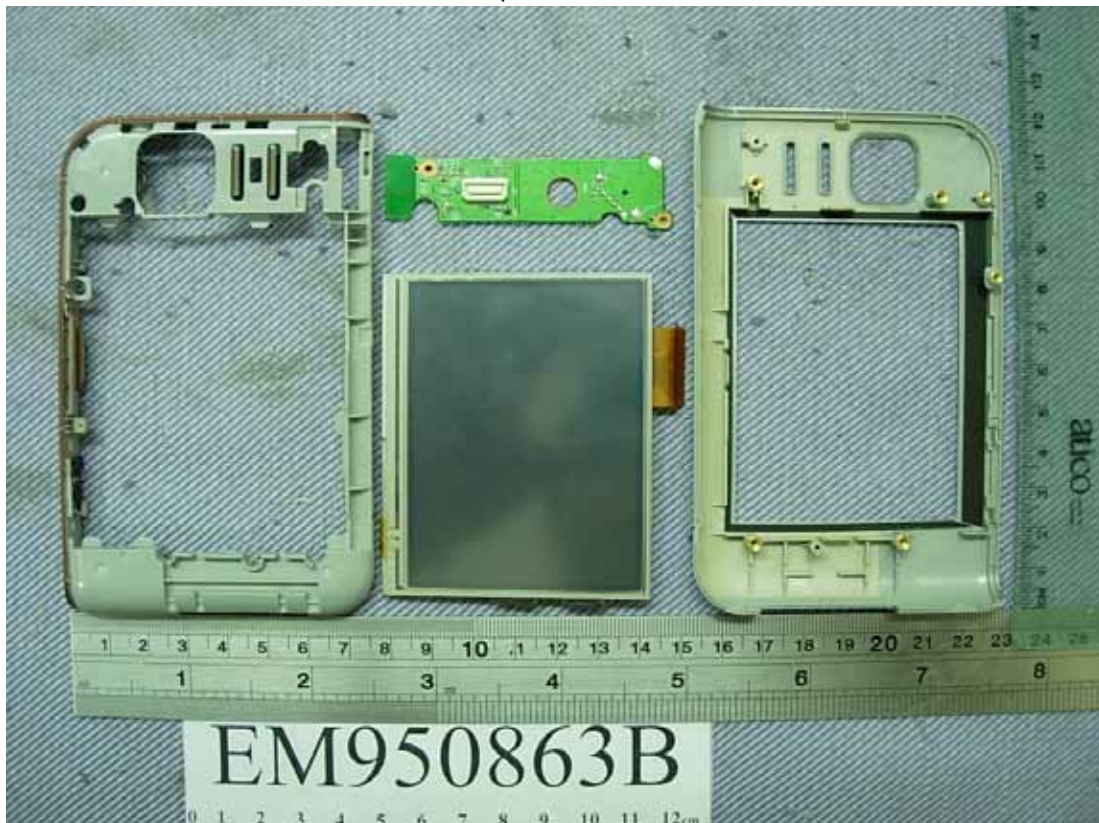
Figure 18 Internal View (Removed Covers, LCD Panel & Bluetooth Board)
