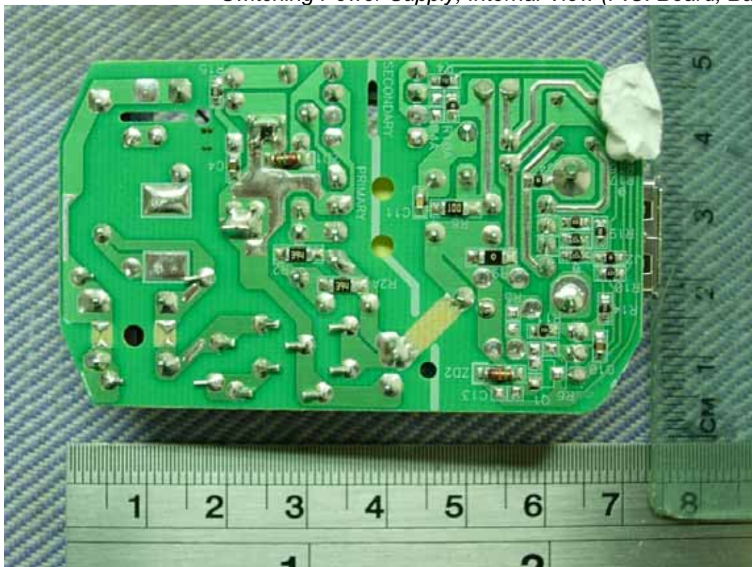
Figure 25 Switching Power Supply, Internal View (P.C. Board, Back View)
