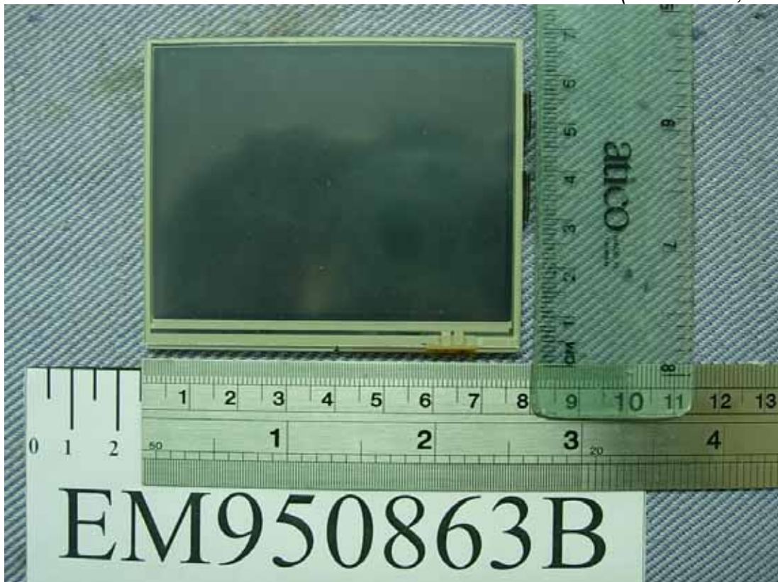
Figure 22 Internal View (LCD Panel, Front View)
