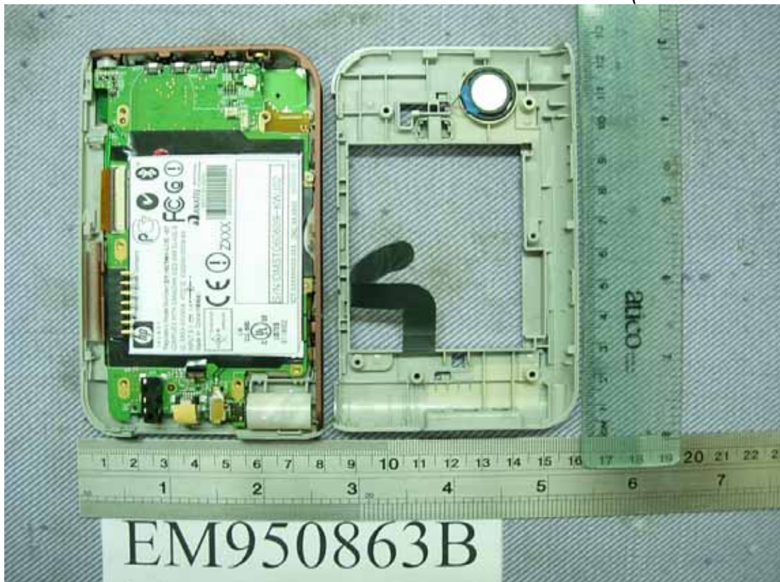
Figure 14 Internal View (Removed Back Cover)
