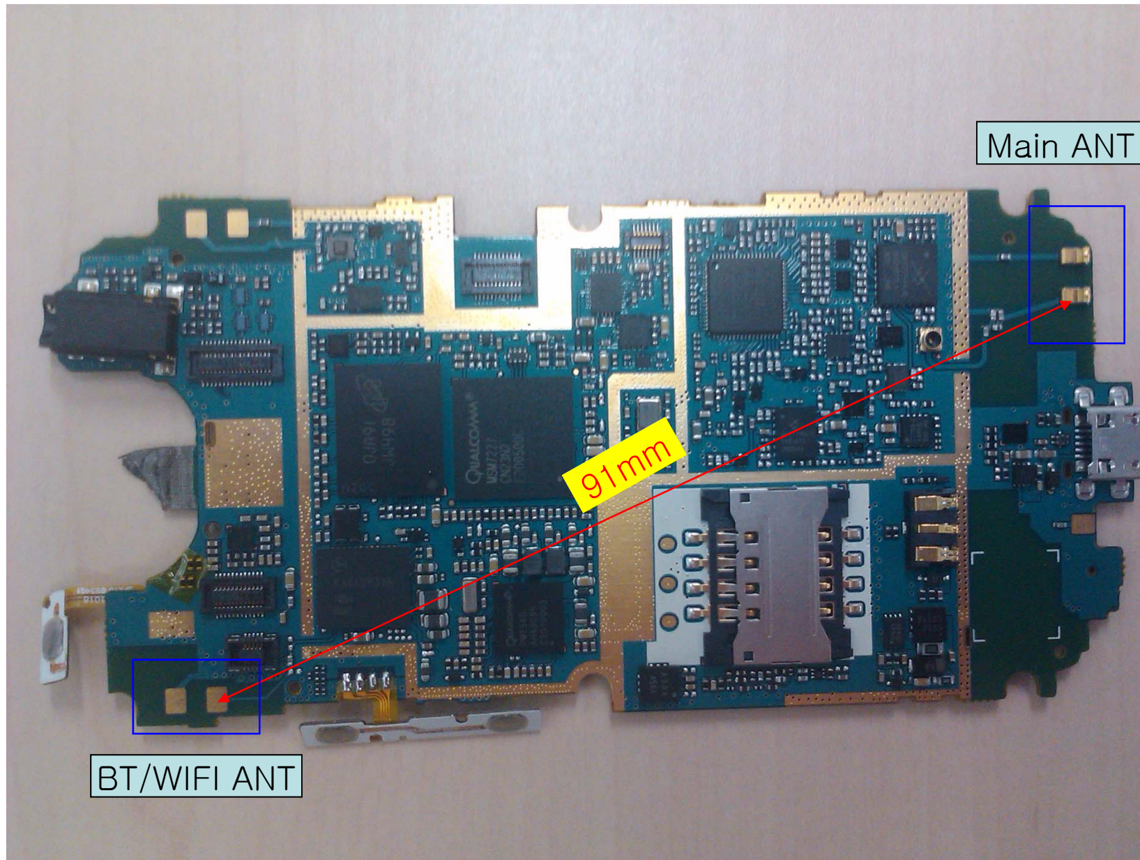
The distance between Main and BT/WIFI ANT
