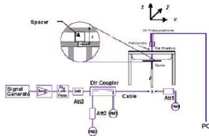
Figure 9.1 Dipole Verification Test Setup Diagram & Photo
