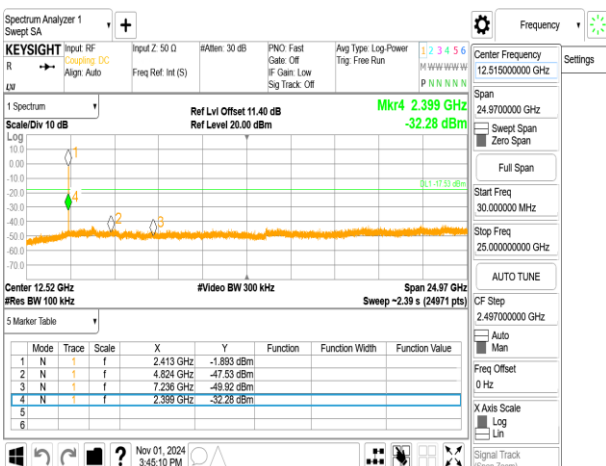
802.11ax_20MHz_ChainA_2412MHz
