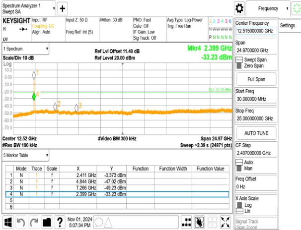
802.11ax_40MHz_ChainA_2422MHz_RU242_61
