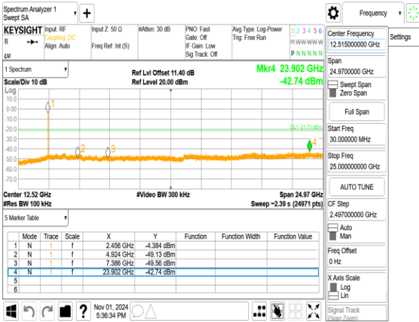
802.11ax_40MHz_ChainA_2462MHz_RU242_62
