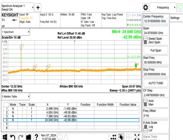
802.11ax_20MHz_ChainA_2462MHz_RU106_54
