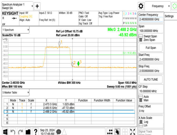
802.11g_20MHz_ChainA_2472MHz
