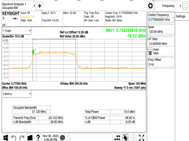
802.11ax_80MHz_ChainA_5775MHz_RU484_65
