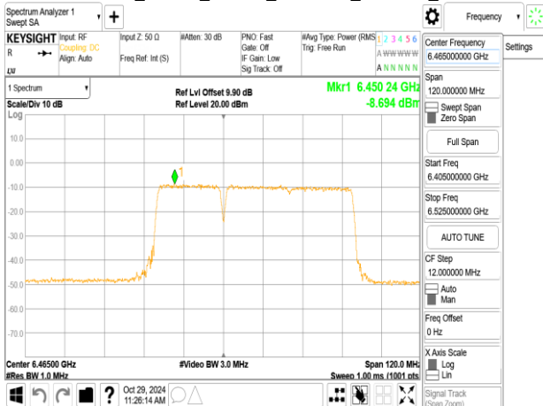
802.11be_80MHz_ChainA_6465MHz_484+242_MRU1
