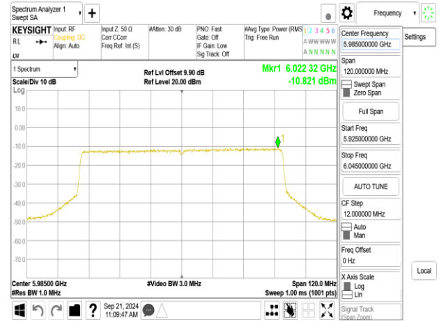
802.11be_80MHz_ChainA_5985MHz_484+242_MRU2
