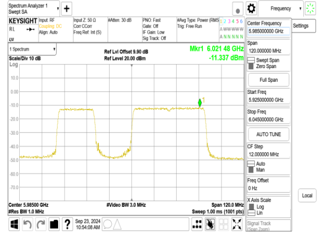
802.11be_80MHz_ChainA_5985MHz_484+242_MRU2
