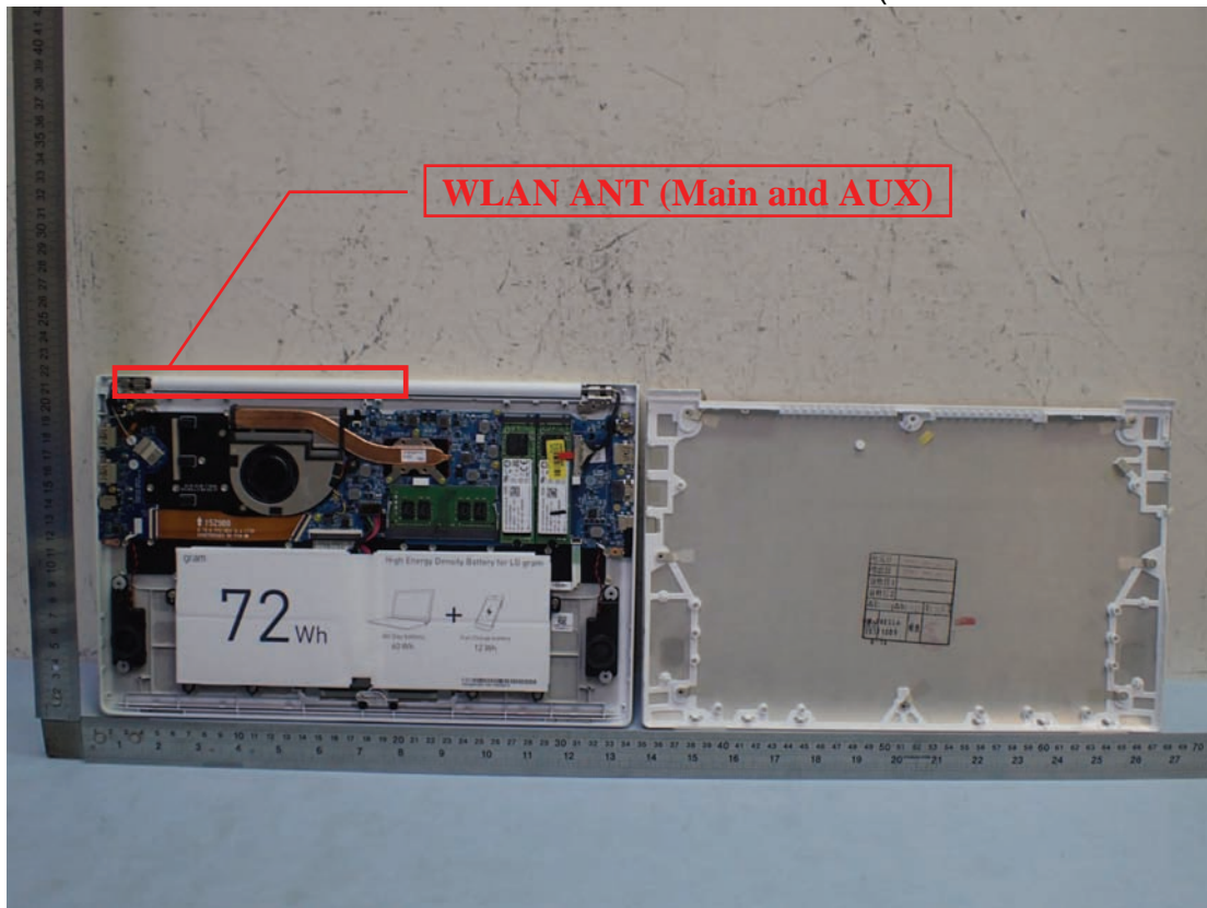
Figure 7 Internal View (Remove Cover View)
