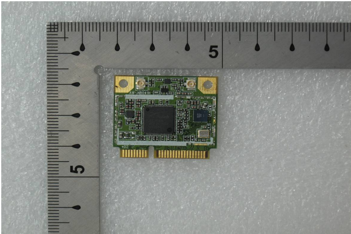
Internal View of EUT – 3 (WLAN /BT Module)
